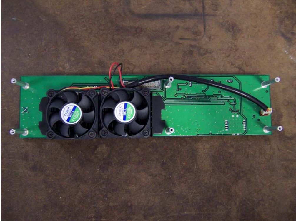
TX PCB - Solder Side
