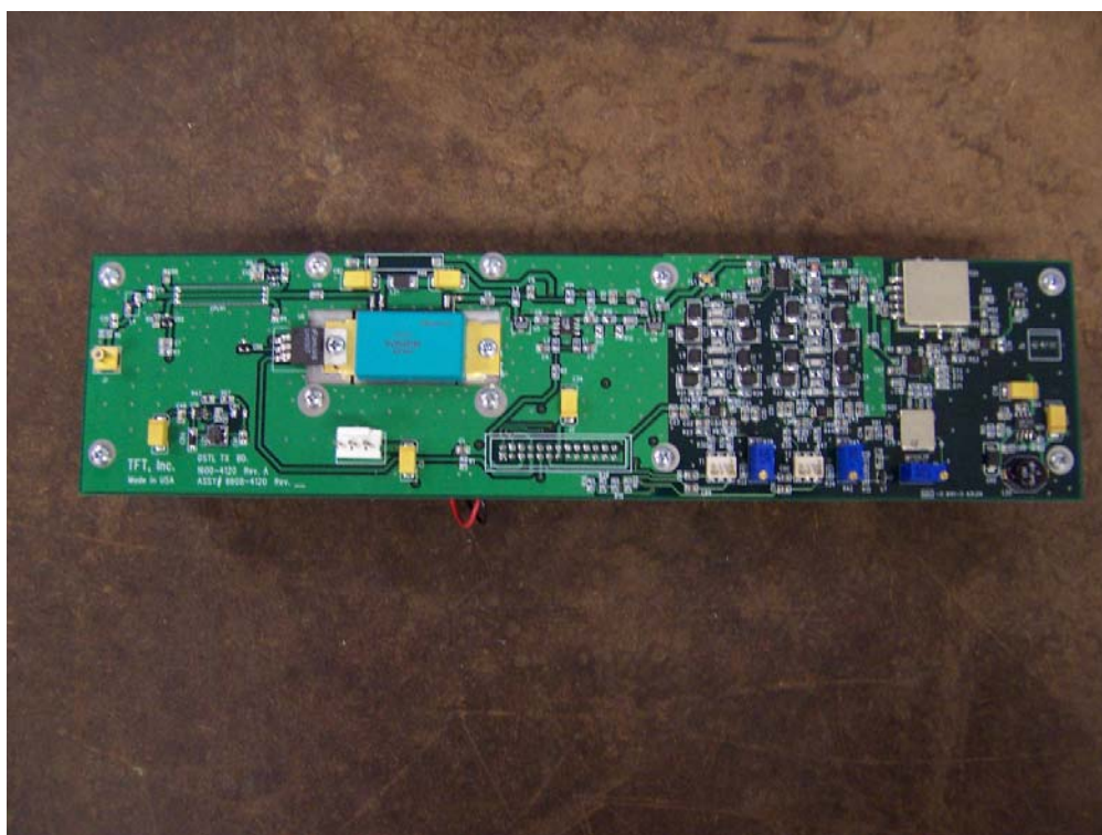
TX PCB – Component Side
