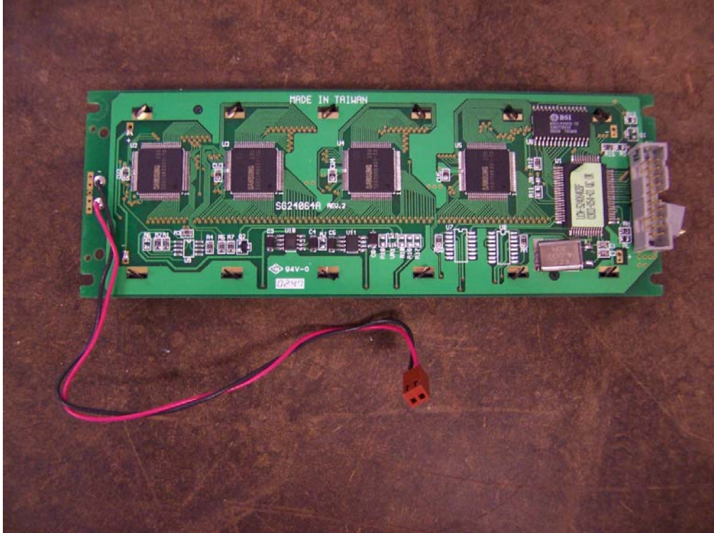
Display PCB – Solder Side
