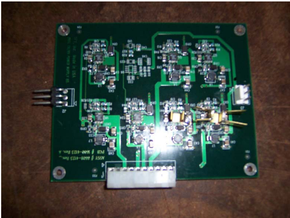
P/S PCB – Component Side
