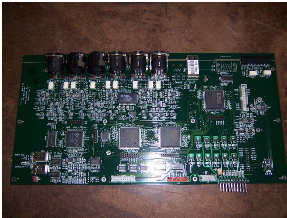
Main PCB – Component Side
