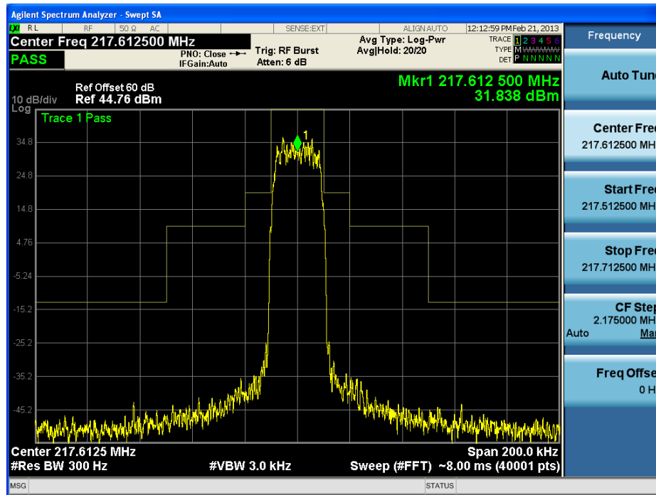
Low Channel = 217.6125 MHz, Full Rate, Max Power
