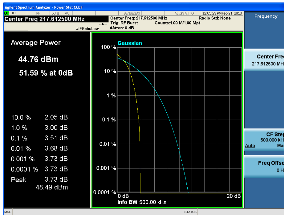
CCDF Average and Peak Power Plot for First Table Entry
