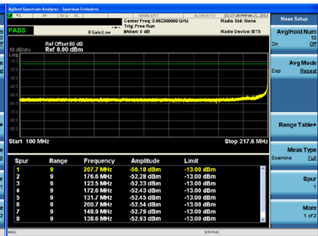
Figure 8C2. 100 to 217.6 MHz, 10 kHz BW
