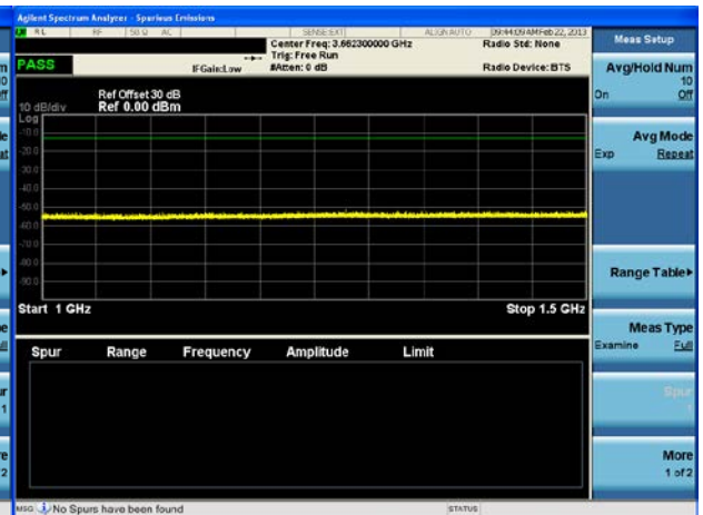
Figure 8C8 1 to 1.5 GHz, 1 MHz BW
