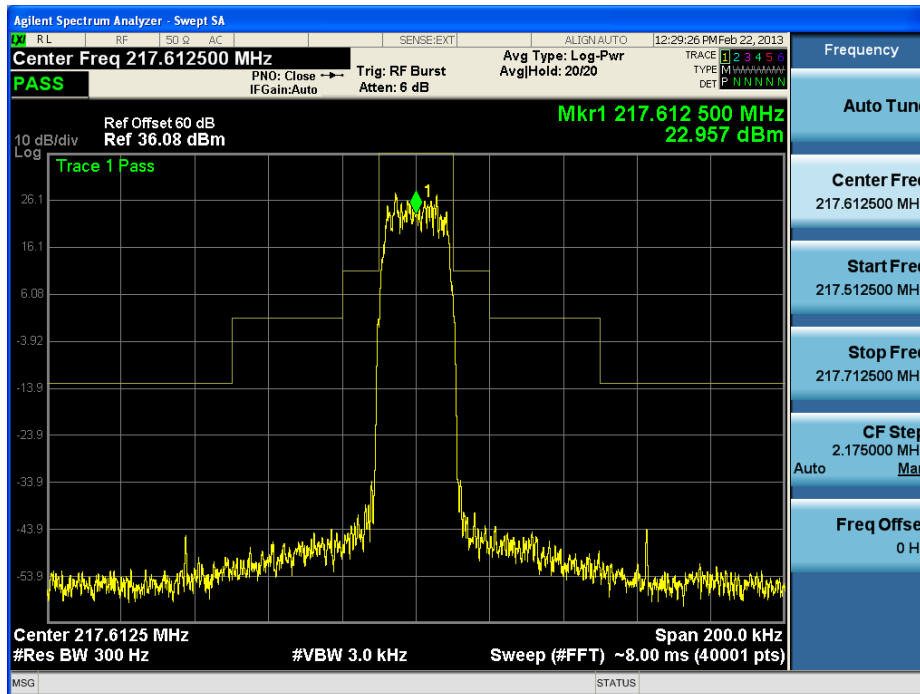
Low Channel = 217.6125 MHz, Full Rate, Min Power
