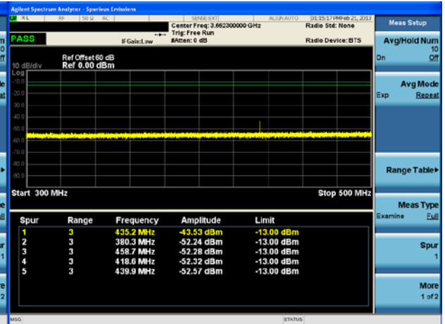
Figure 8C6 300 to 500 MHz, 10kHz BW
