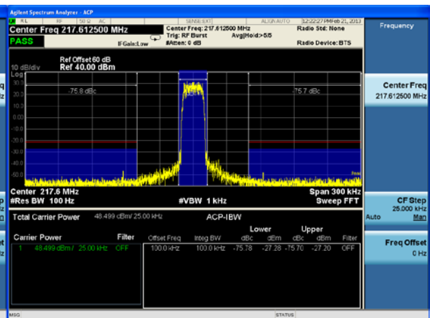
Figure 8C4. fo ± 150 kHz, 100kHz IBW
