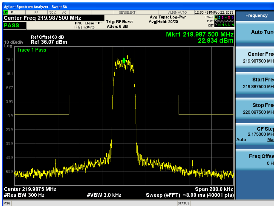
High Channel = 219.9875 MHz, Full Rate, Min Power
