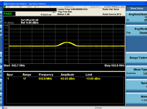
Figure 8C12, Zoom 3xfo, 652.8 MHz
