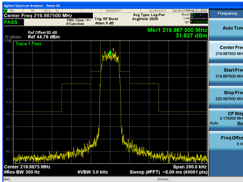
High Channel = 219.9875 MHz, Full Rate, Max Power
