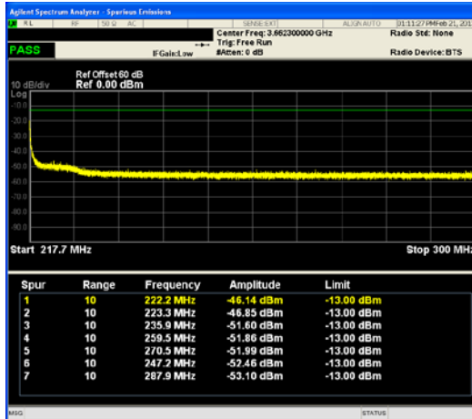
Figure 8C5 217 to 300 MHz, 10kHz BW
