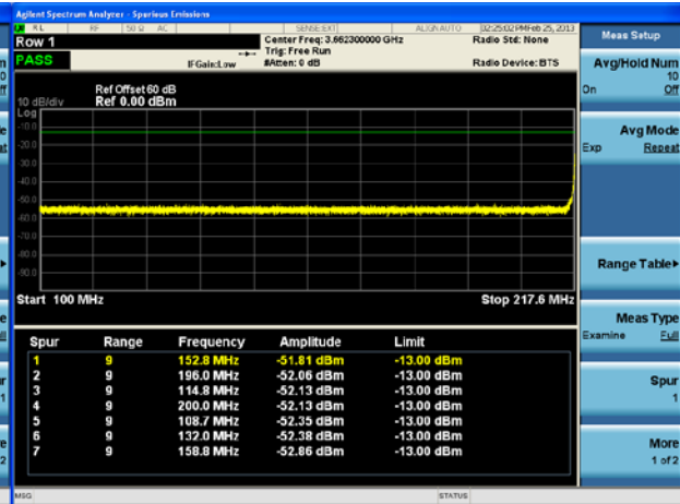
Figure 8C2. 100 to 217.6 MHz, 10 kHz BW
