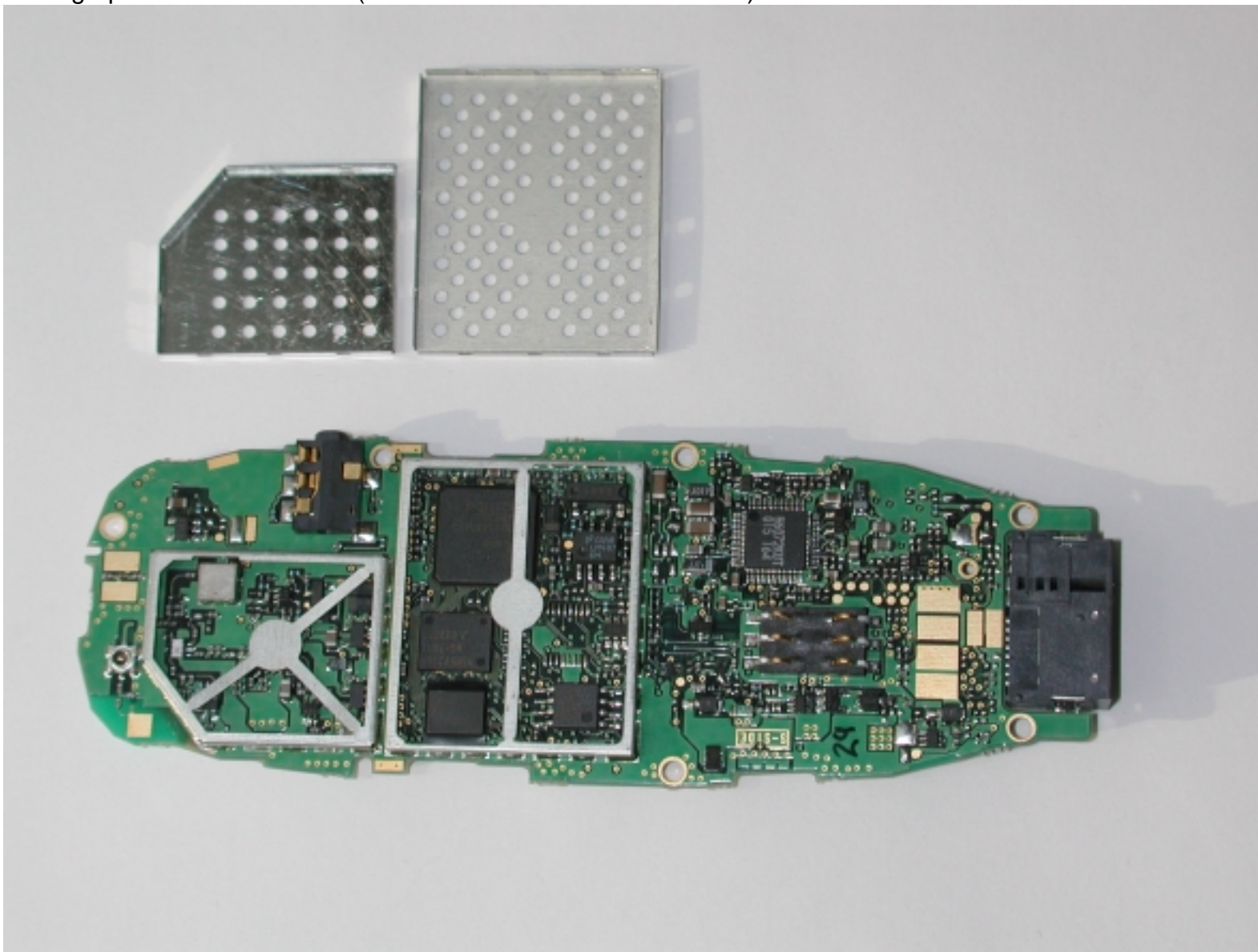
Photograph 7 MT289XG01A (Back PWB with Shields Removed)
