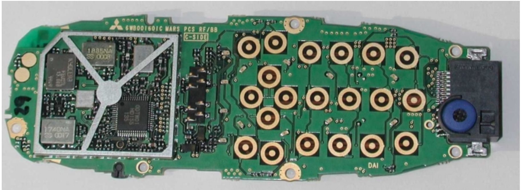
Photograph 8 MT289XG01A (Front PWB without Shield)
