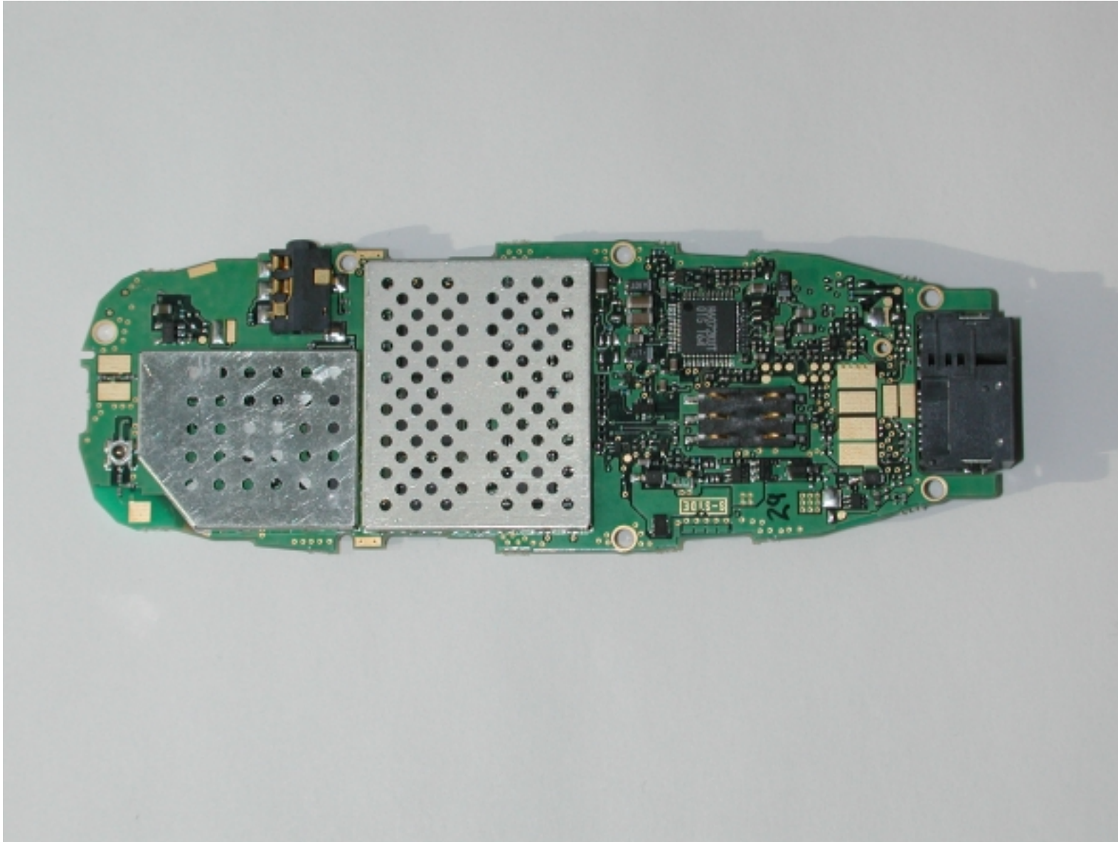
Photograph 6 MT289XG01A (Back PWB with Shields)
