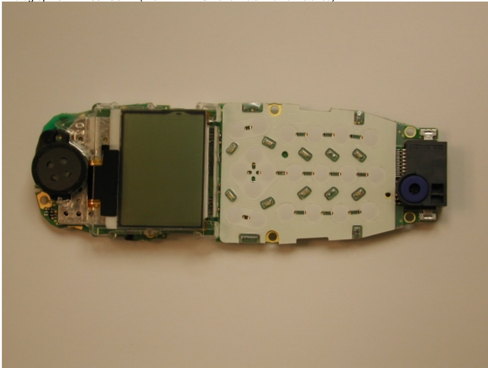
Photograph 3 MT289XG01A (Front PWB LCD and Metal Dome Installed)
