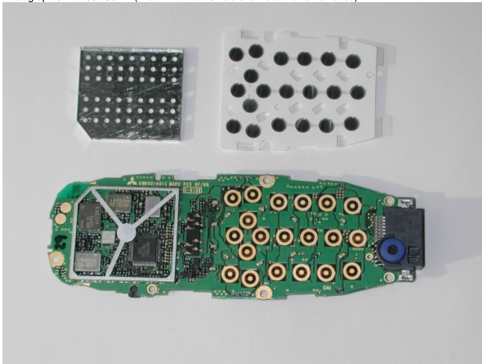
Photograph 5 MT289XG01A (Front PWB with Shield and Metal Dome Removed)
