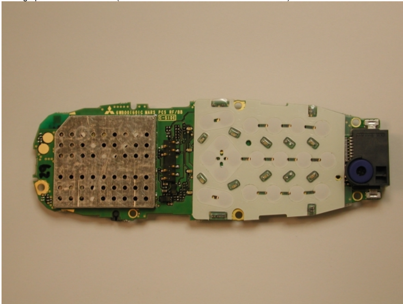
Photograph 4 MT289XG01A (Front PWB with Shield Cover and Metal Dome)
