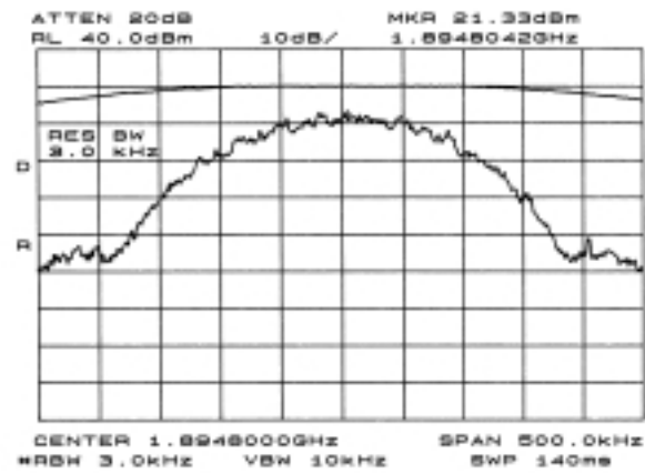
Figure 6.5.5 Lower and Upper Band Edges of Block F
