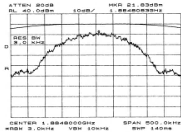
Figure 6.5.3 Lower and Upper Band Edges of Block B
