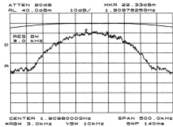
Figure 6.5.6 Lower and Upper Band Edges of Block C
