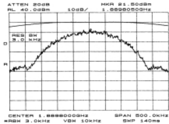
Figure 6.5.4 Lower and Upper Band Edges of Block E
