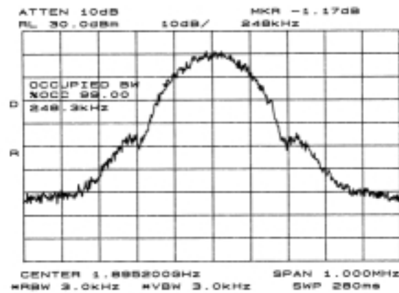
Figure 6.4.11 Block C Lower Edge 99% Power Occupied Bandwidth (Ch 737)
