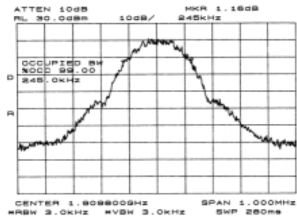
Figure 6.4.12 Block C Upper Edge 99% Power Occupied Bandwidth (Ch 810)
