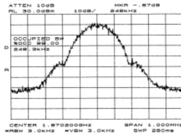
Figure 6.4.5 Block B Lower Edge 99% Power Occupied Bandwidth (Ch 612)
