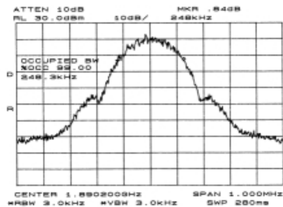
Figure 6.4.9 Block F Lower Edge 99% Power Occupied Bandwidth (Ch 712)
