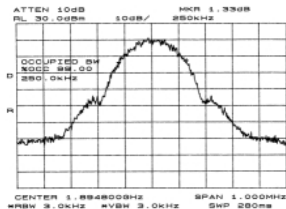
Figure 6.4.10 Block F Upper Edge 99% Power Occupied Bandwidth (Ch 735)
