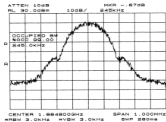
Figure 6.4.6 Block B Upper Edge 99% Power Occupied Bandwidth (Ch 685)
