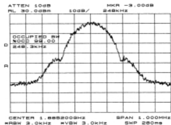
Figure 6.4.7 Block E Lower Edge 99% Power Occupied Bandwidth (Ch 687)
