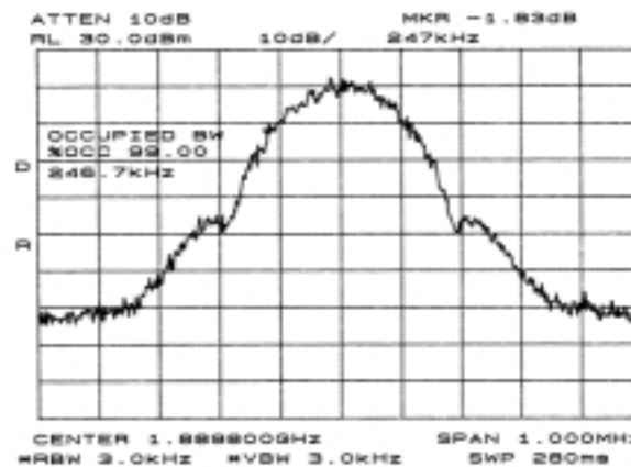
Figure 6.4.8 Block E Upper Edge 99% Power Occupied Bandwidth (Ch 710)
