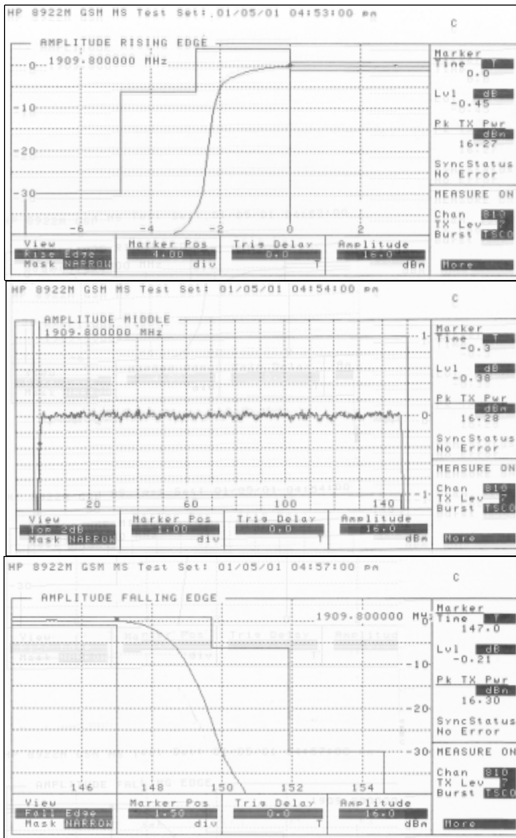
Figure 6.2.8 Carrier 1909.8 MHz (Ch 810) Power Level 7
