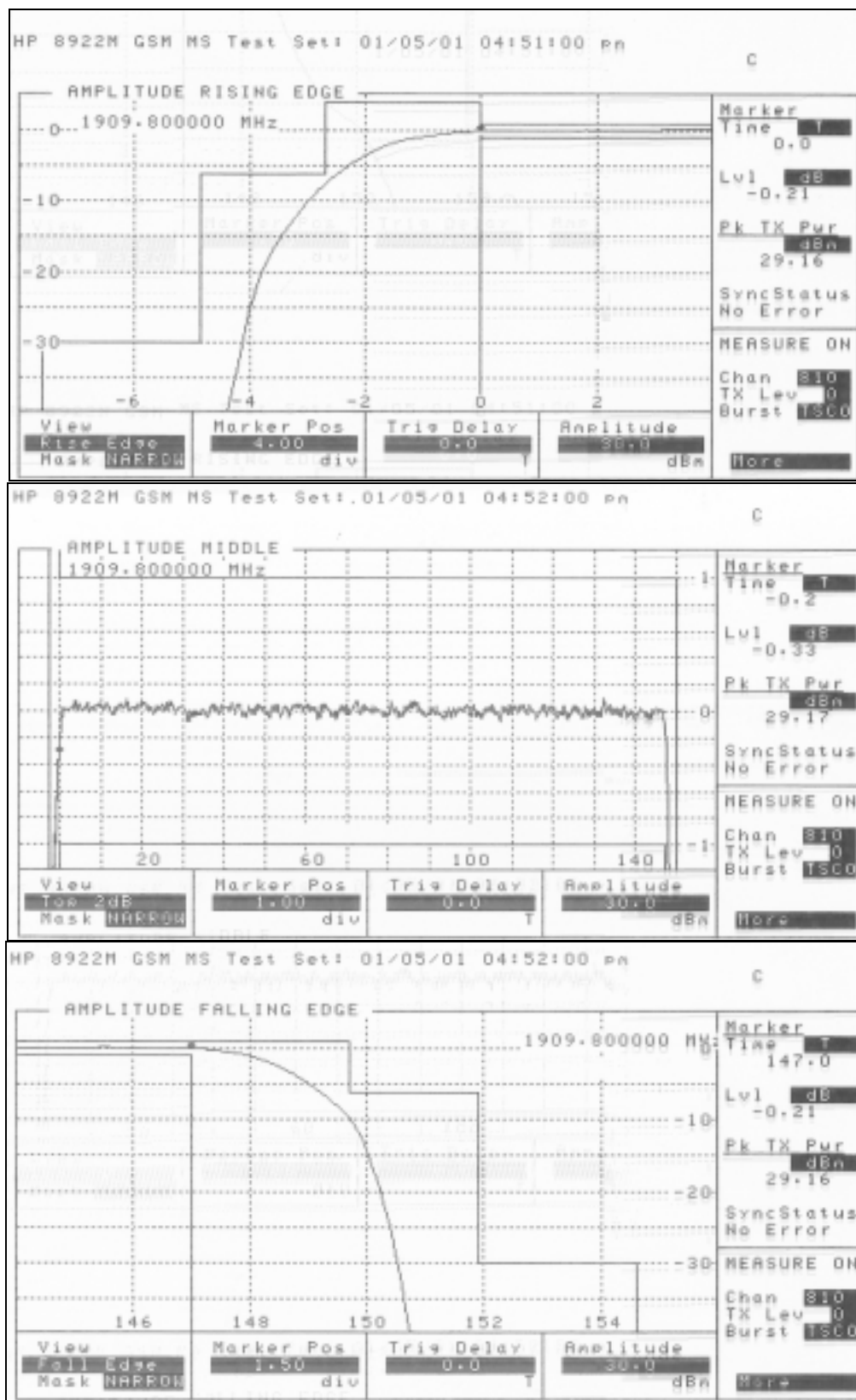
Figure 6.2.7 Carrier 1909.8 MHz (Ch 810) Power Level 0
