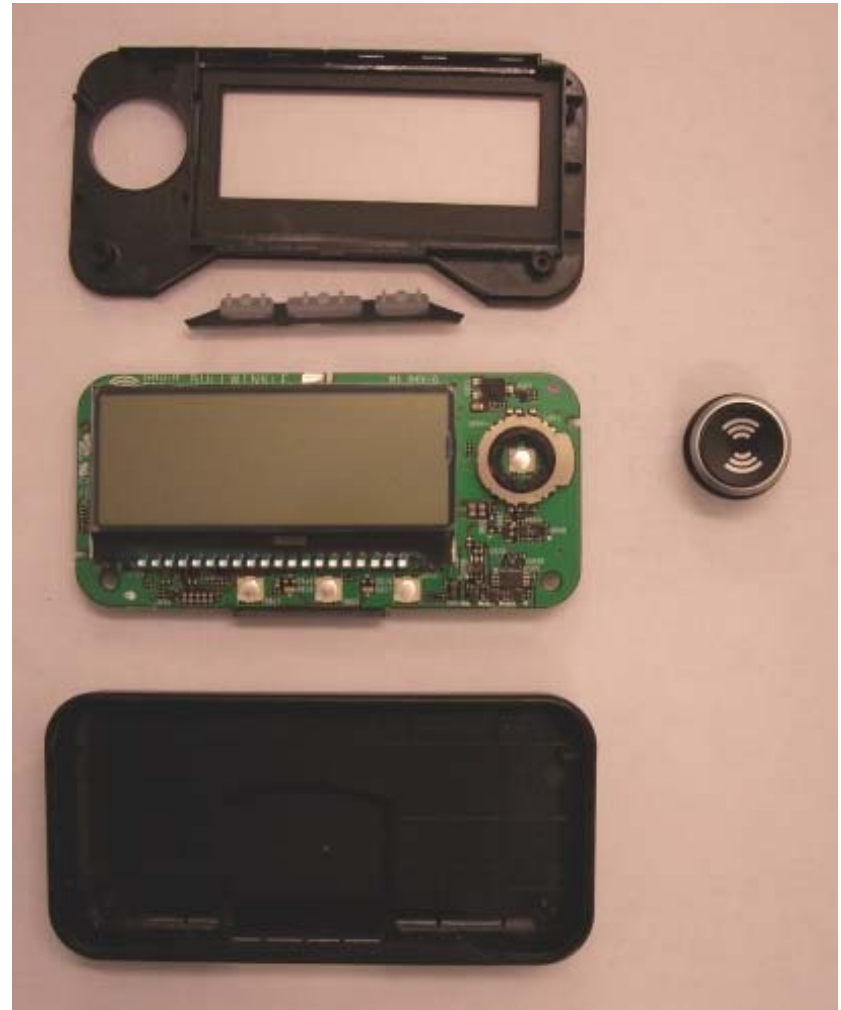
Open Case with PCB removed
