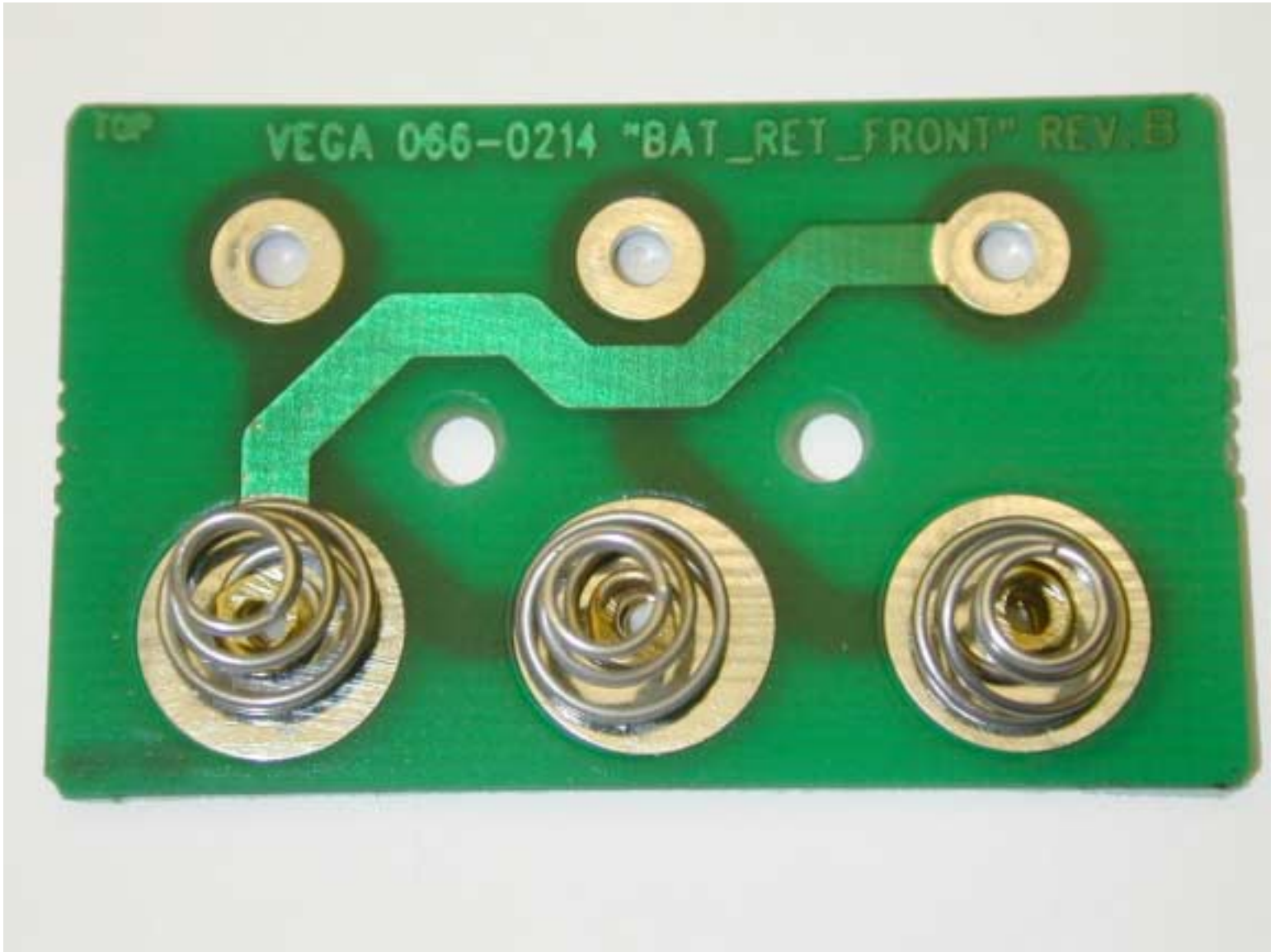
BATTERY RETAINER #2 CONTACT SIDE
