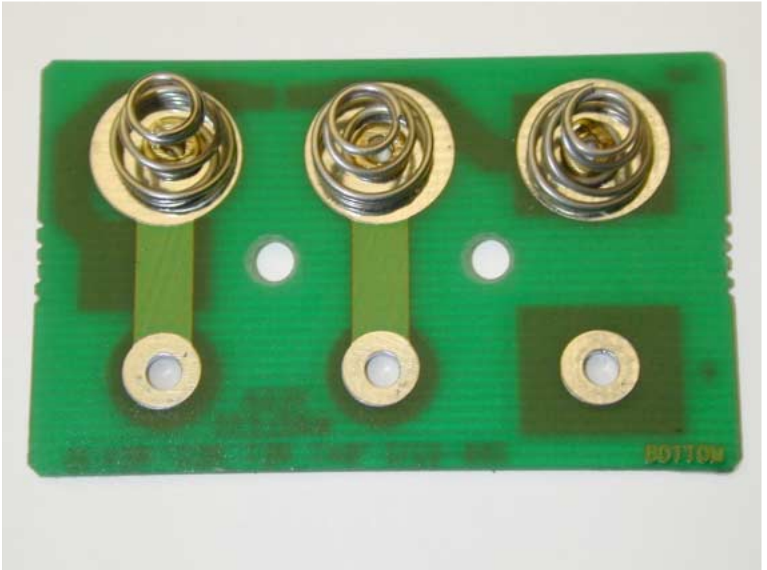
BATTERY RETAINER #1 BATTERY CONTACT SIDE
