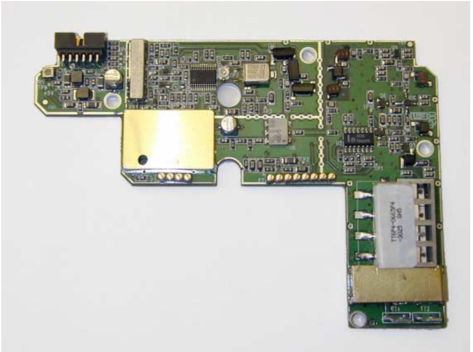
Transmitter rf TOP COMPONENT SIDE WITH SHIELD
