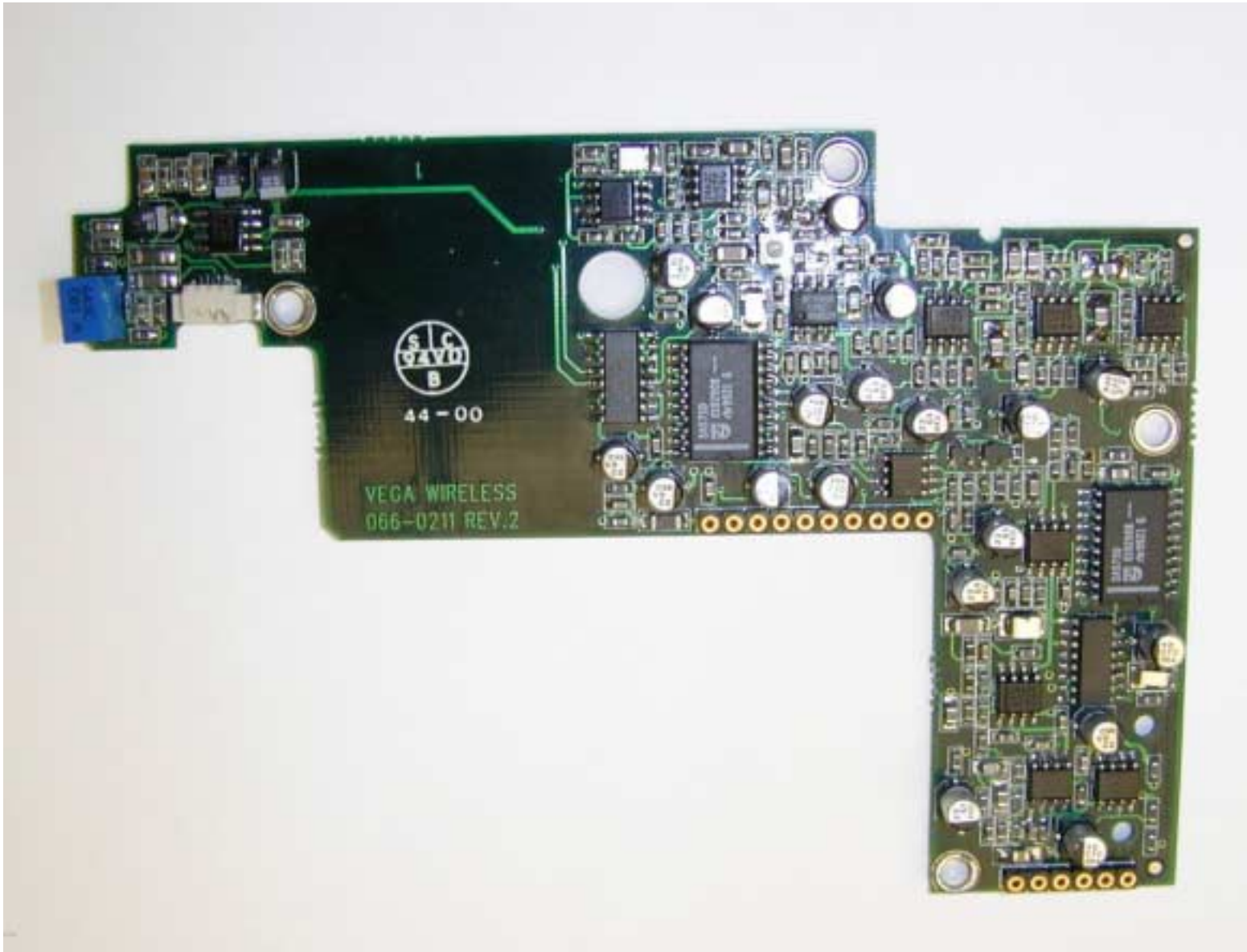
Rceiver AUDIO TOP, Component side
