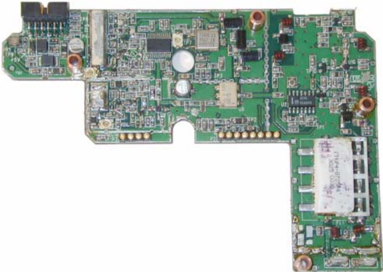
Transmitter top, component side without shield
