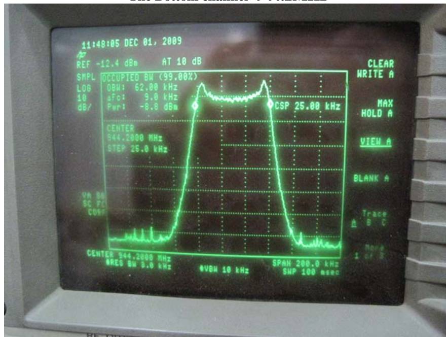
The Bottom channel -944.2MHz
