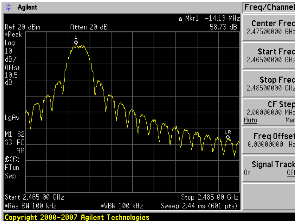
BandEdge (CH 24)
