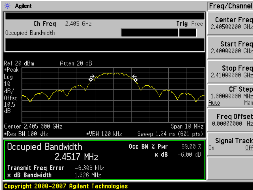
6dB Bandwidth plot (CH 11)
