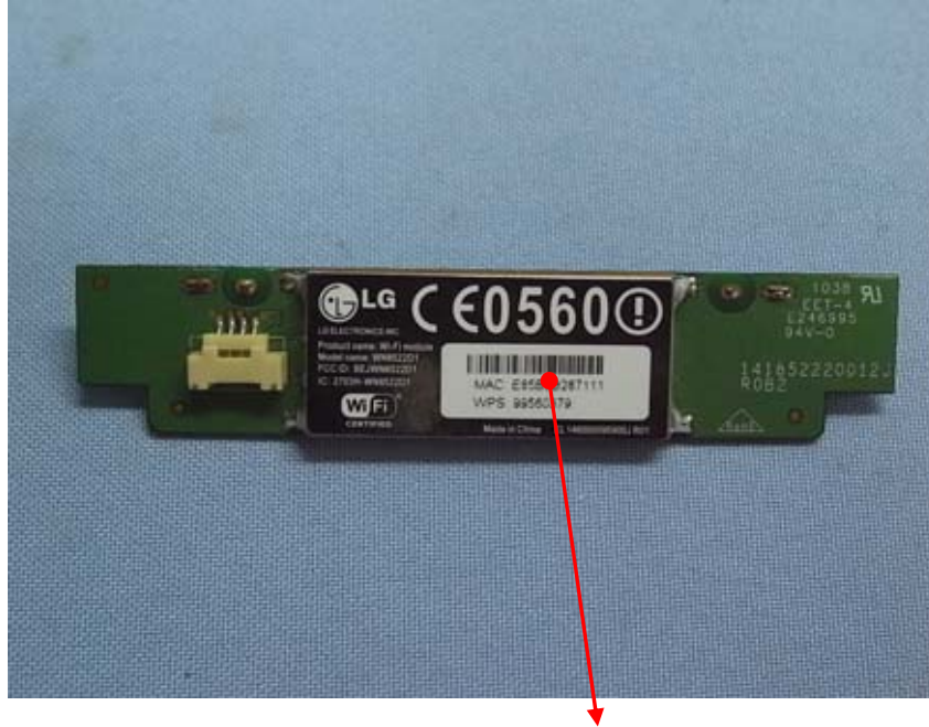
FCC Label Placement Location
