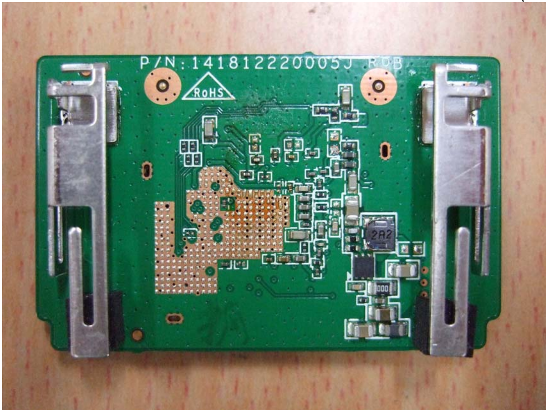
Figure 3 Wi-Fi module (Back View)
