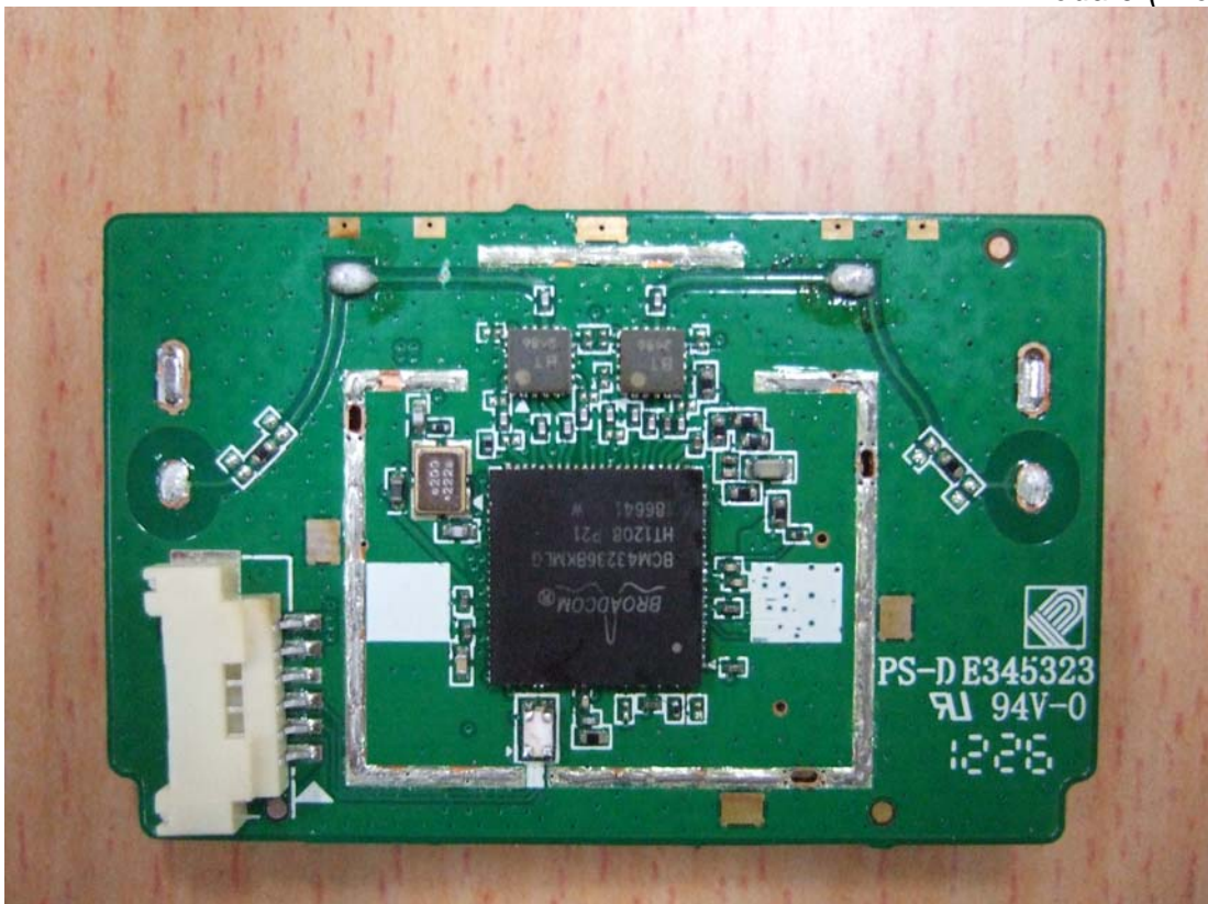
Figure 2 Wi-Fi module (Front View)
