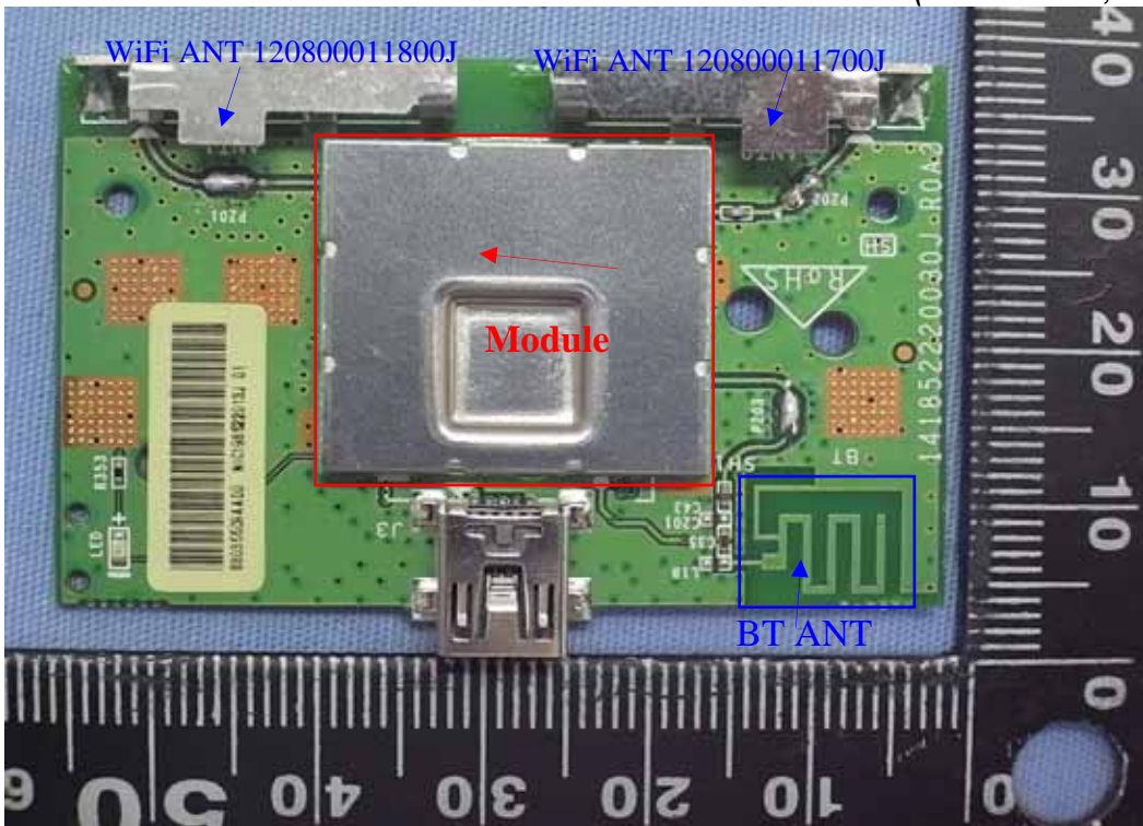
Figure 8 Internal View (Main Board, Front View)
