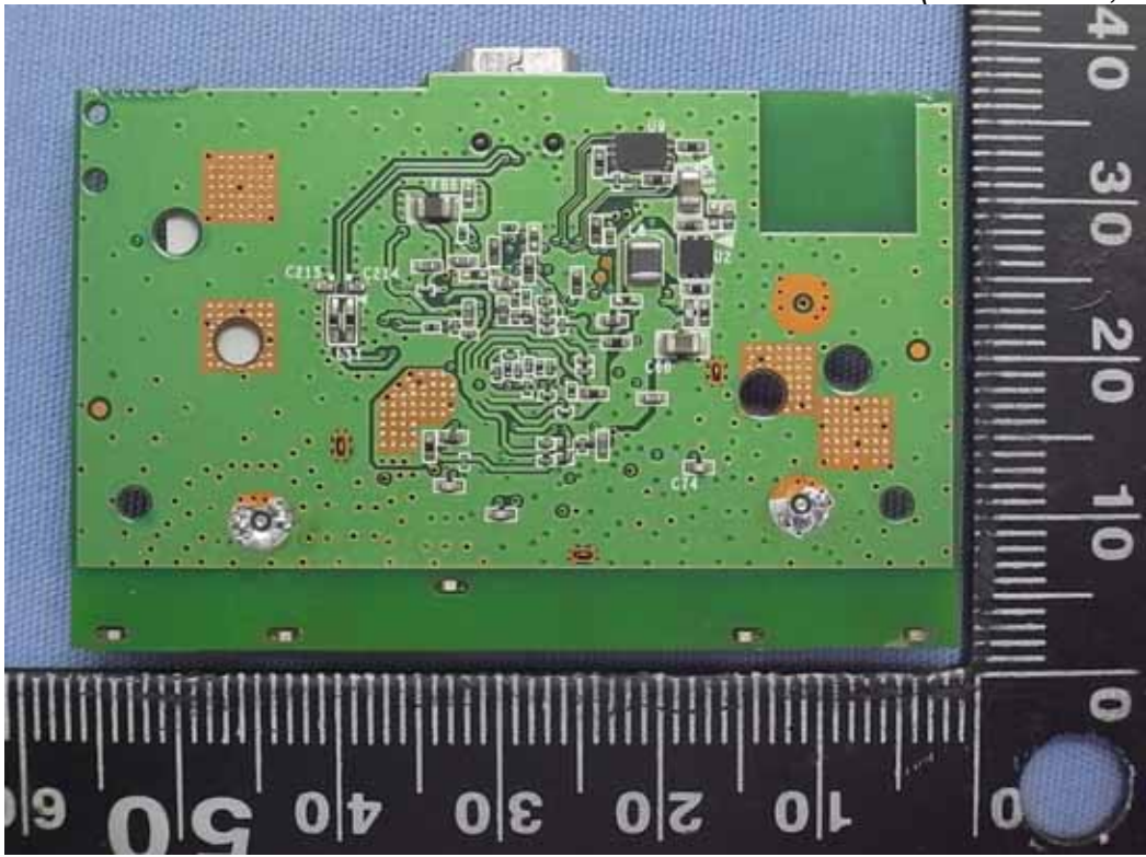
Figure 10 Internal View (Main Board, Removed Shielded Cover)
