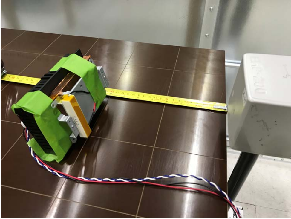
E/H Field Measurement on EUT Side "E"
