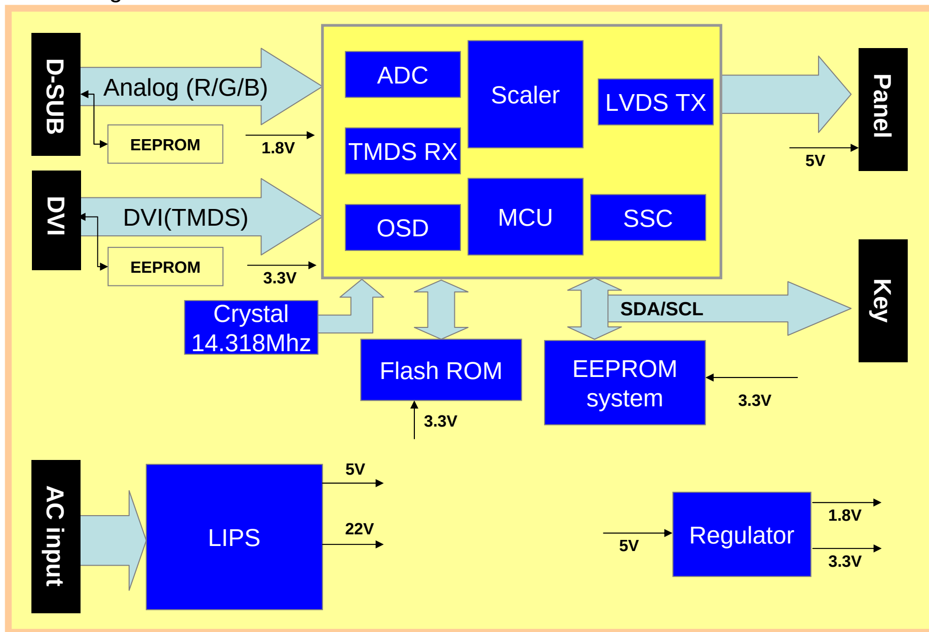
Block diagram
