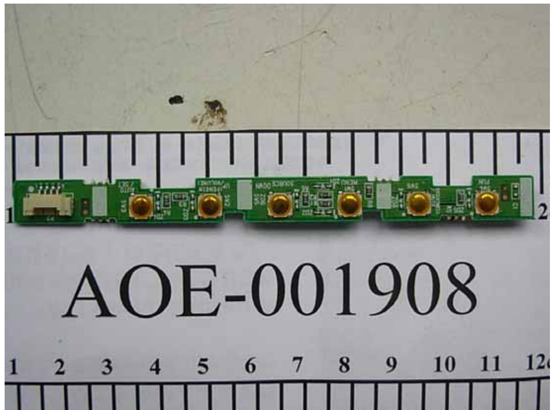
FIGURE 19 LCD MONITOR (M/N: W2252TET) KEY BOARD (COMPONENT SIDE)
