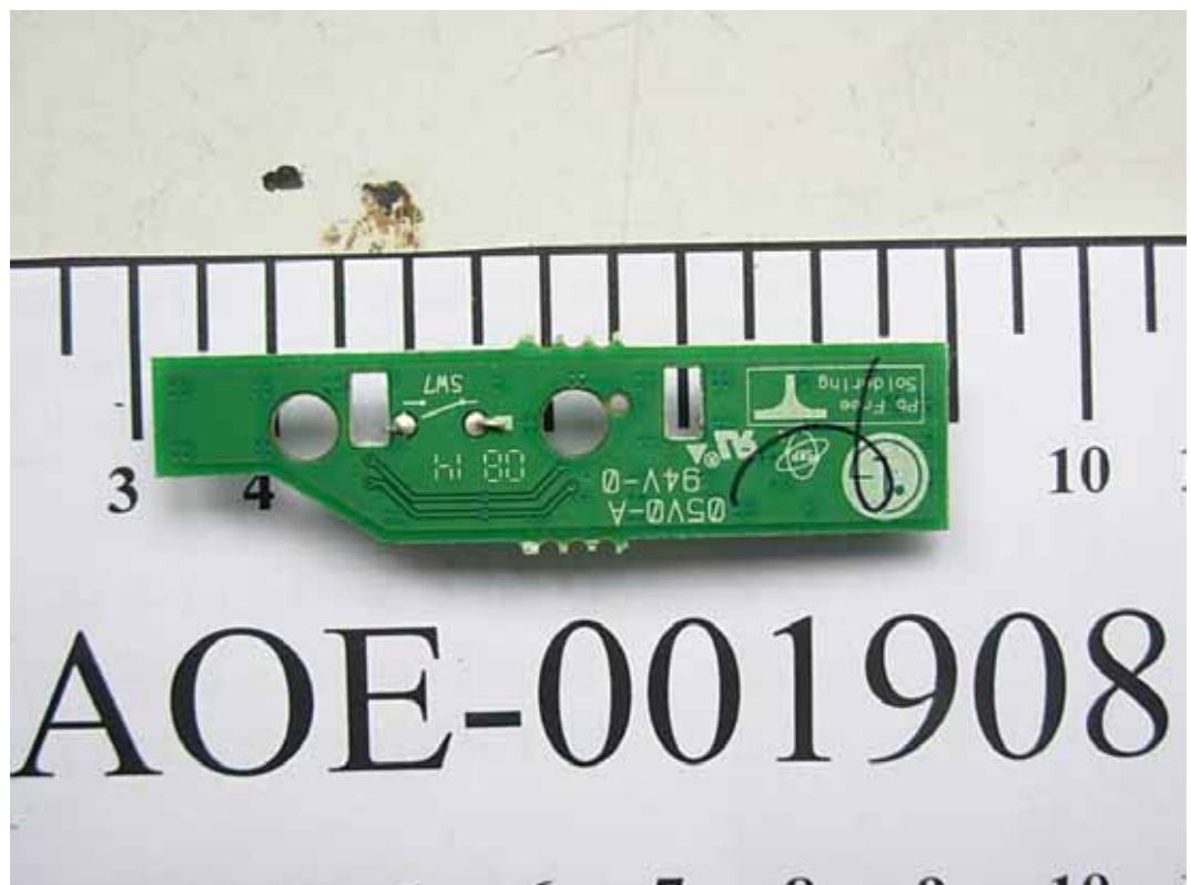
FIGURE 18 LCD MONITOR (M/N: W2252TET) LED BOARD (SOLDERED SIDE)
