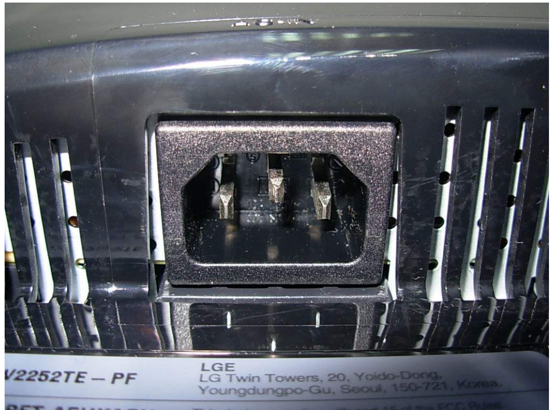
FIGURE 5 LCD MONITOR (M/N: L1742SMT) PORTS 2
