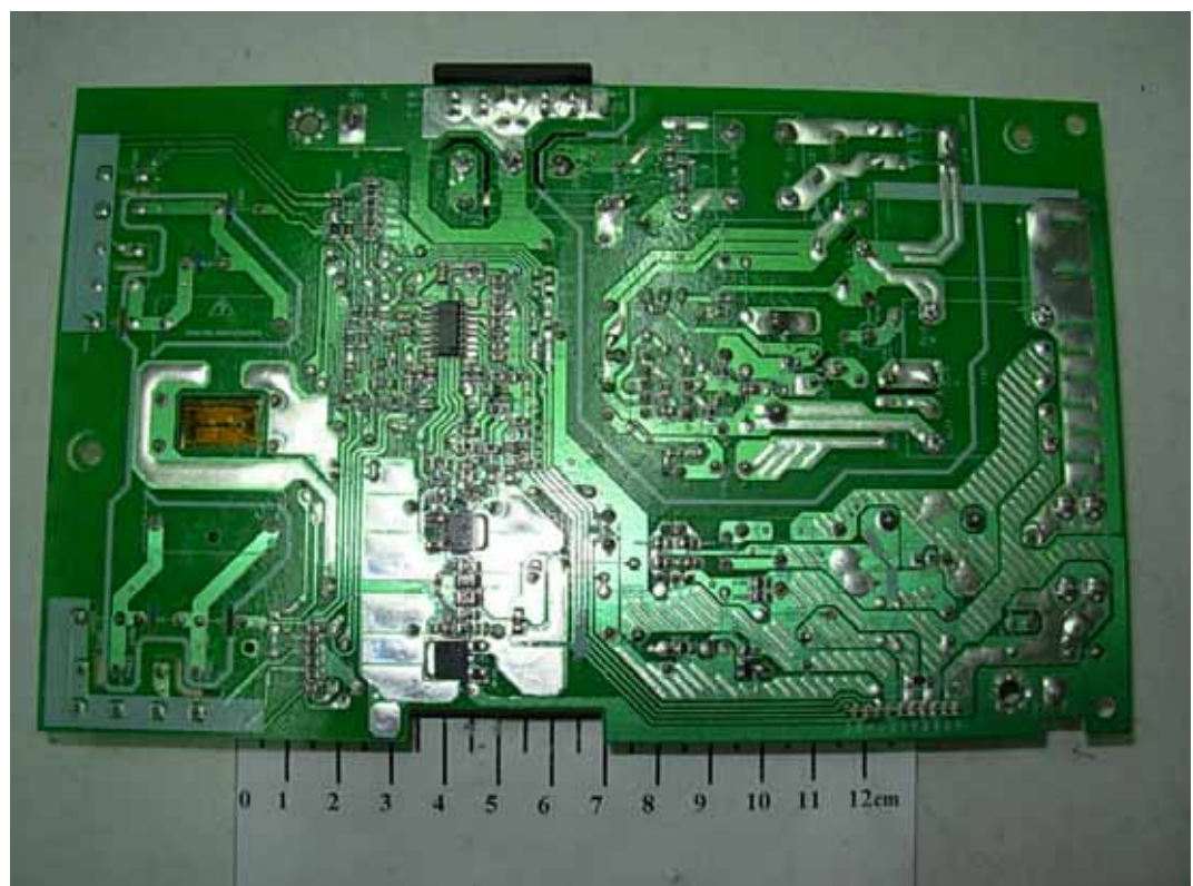
FIGURE 10 LCD MONITOR (M/N: W2244TV) POWER BOARD (SOLDERED SIDE)
