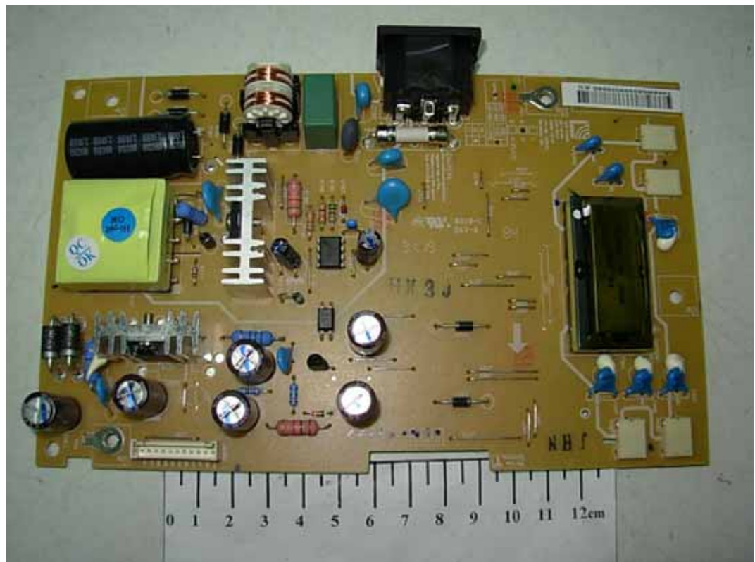
FIGURE 9 LCD MONITOR (M/N: W2244TV) POWER BOARD (COMPONENT SIDE)
