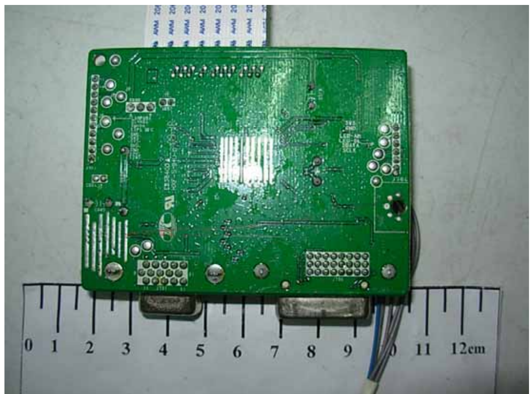
FIGURE 6 LCD MONITOR (M/N: W2244TV) MAIN BOARD (SOLDERED SIDE)
