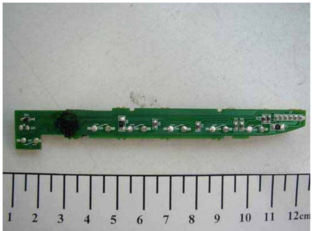
FIGURE 4 LCD MONITOR (M/N: W2243SV) KEYBOARD (SOLDERED SIDE)
