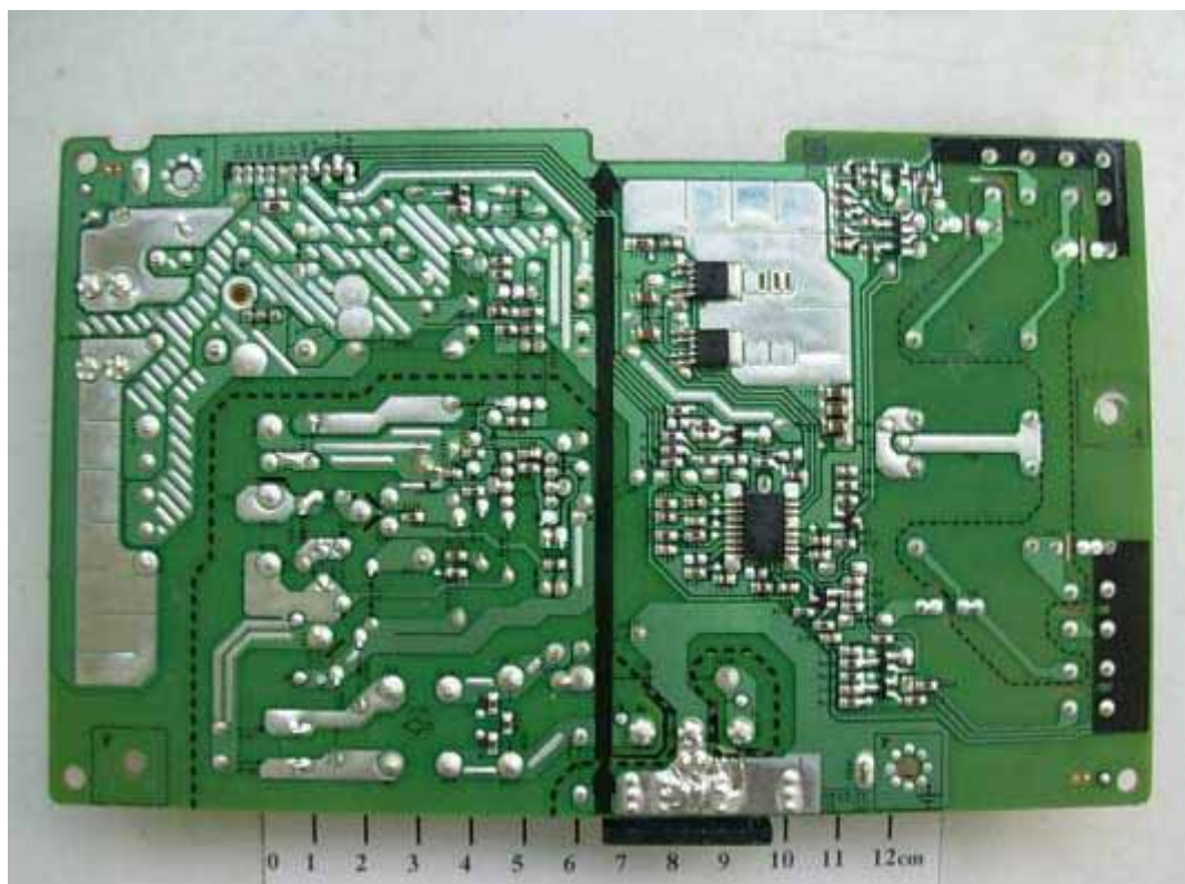
FIGURE 9 LCD MONITOR (M/N: W2243SV) POWER BOARD (SOLDERED SIDE)
