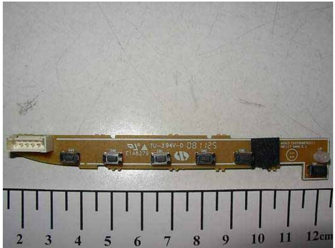
FIGURE 3 LCD MONITOR (M/N: W2243SV) KEYBOARD (COMPONENT SIDE)
