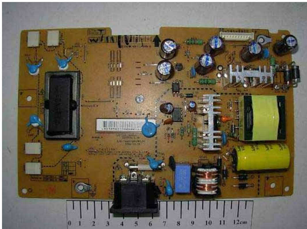
FIGURE 8 LCD MONITOR (M/N: W2243SV) POWER BOARD (COMPONENT SIDE)
