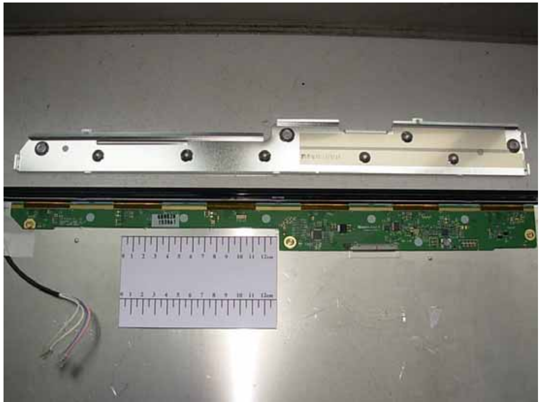
FIGURE 11 LCD MONITOR (M/N: W2240TV) LCD PANEL MAIN BOARD (COMPONENT SIDE)
