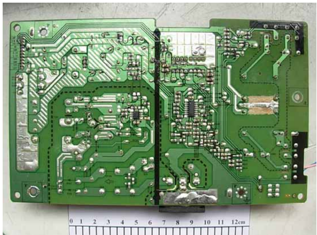
FIGURE 6 LCD MONITOR (M/N: W2240TV) POWER BOARD (SOLDERED SIDE)
