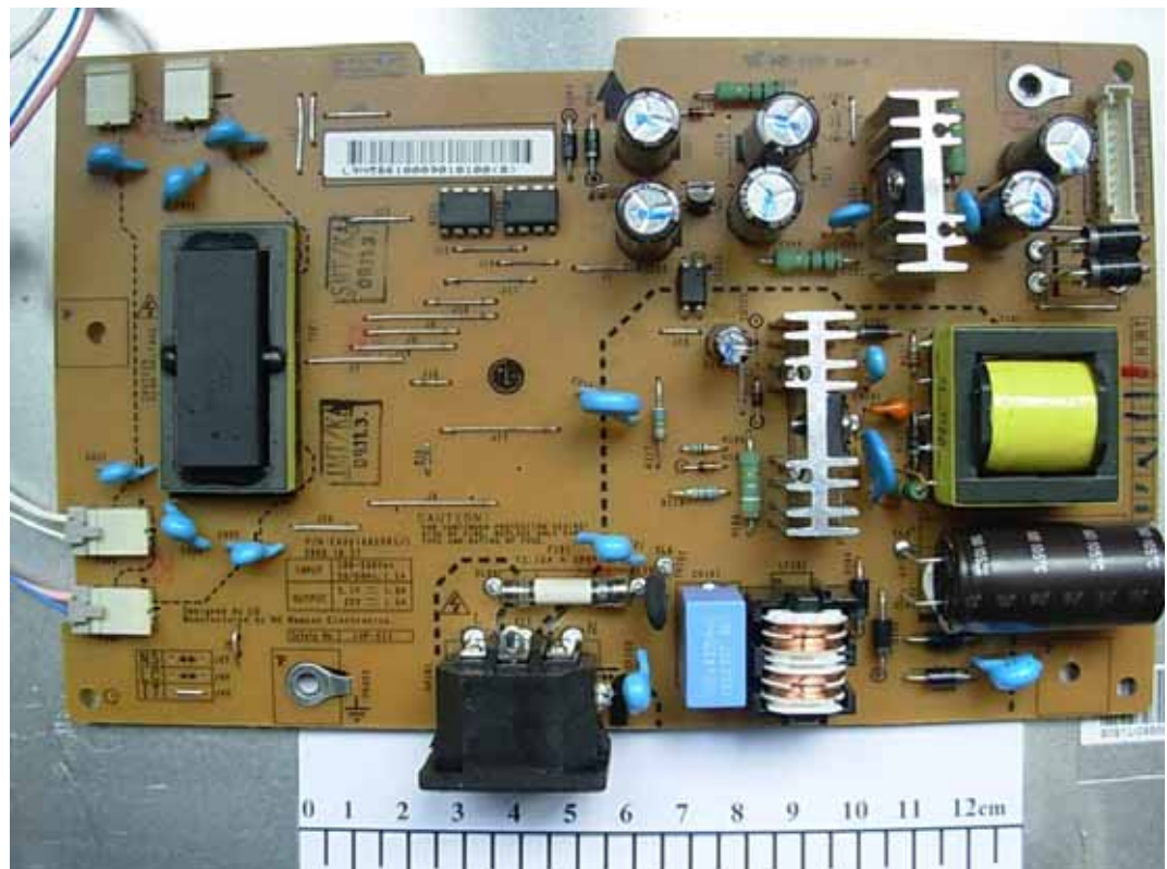
FIGURE 5 LCD MONITOR (M/N: W2240TV) POWER BOARD (COMPONENT SIDE)
