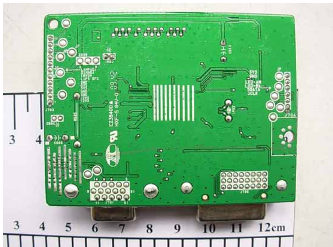
FIGURE 8 LCD MONITOR (M/N: W2240TV) MAIN BOARD (SOLDERED SIDE)
