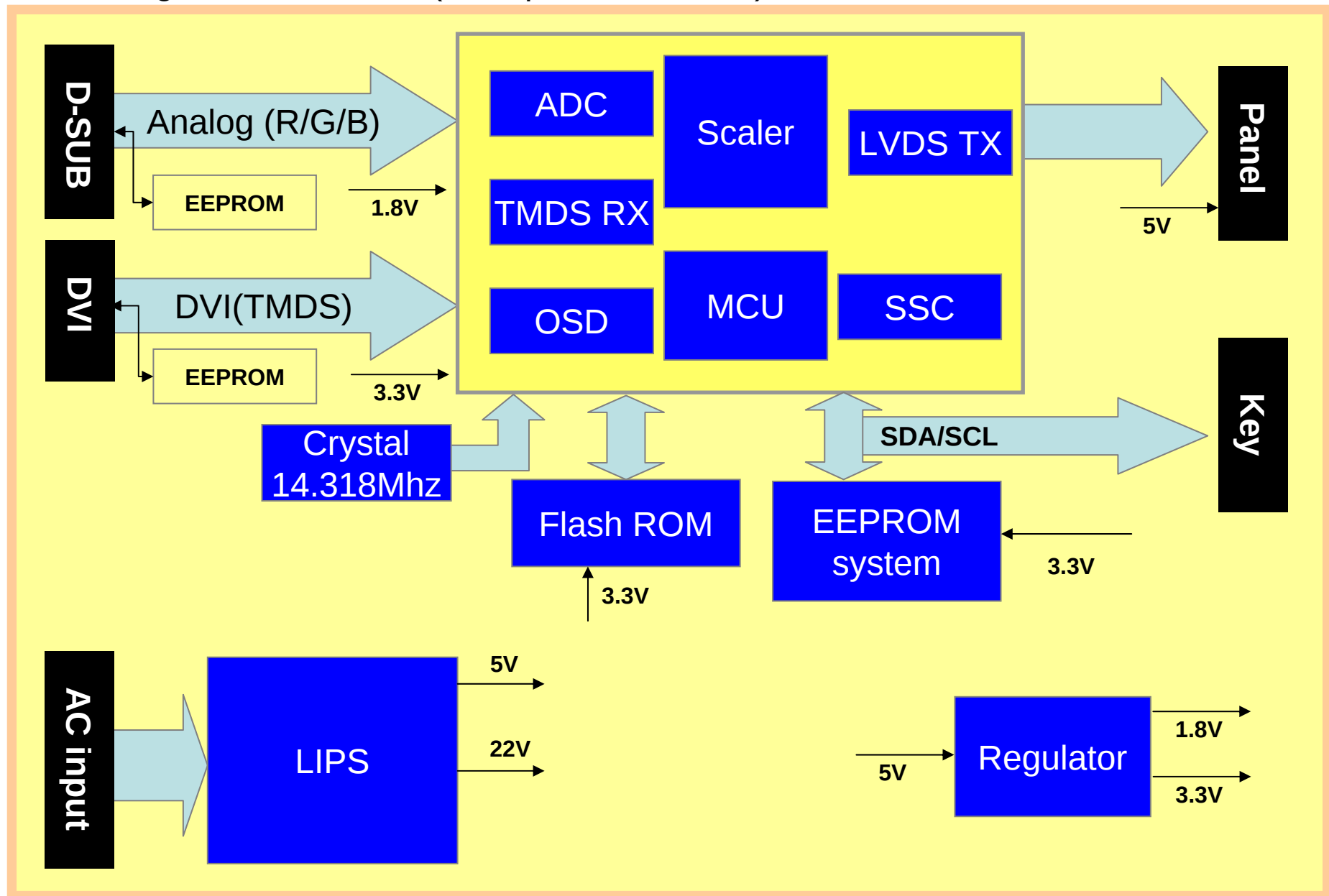
Block diagram for W53/54 ( except HDMI model)
