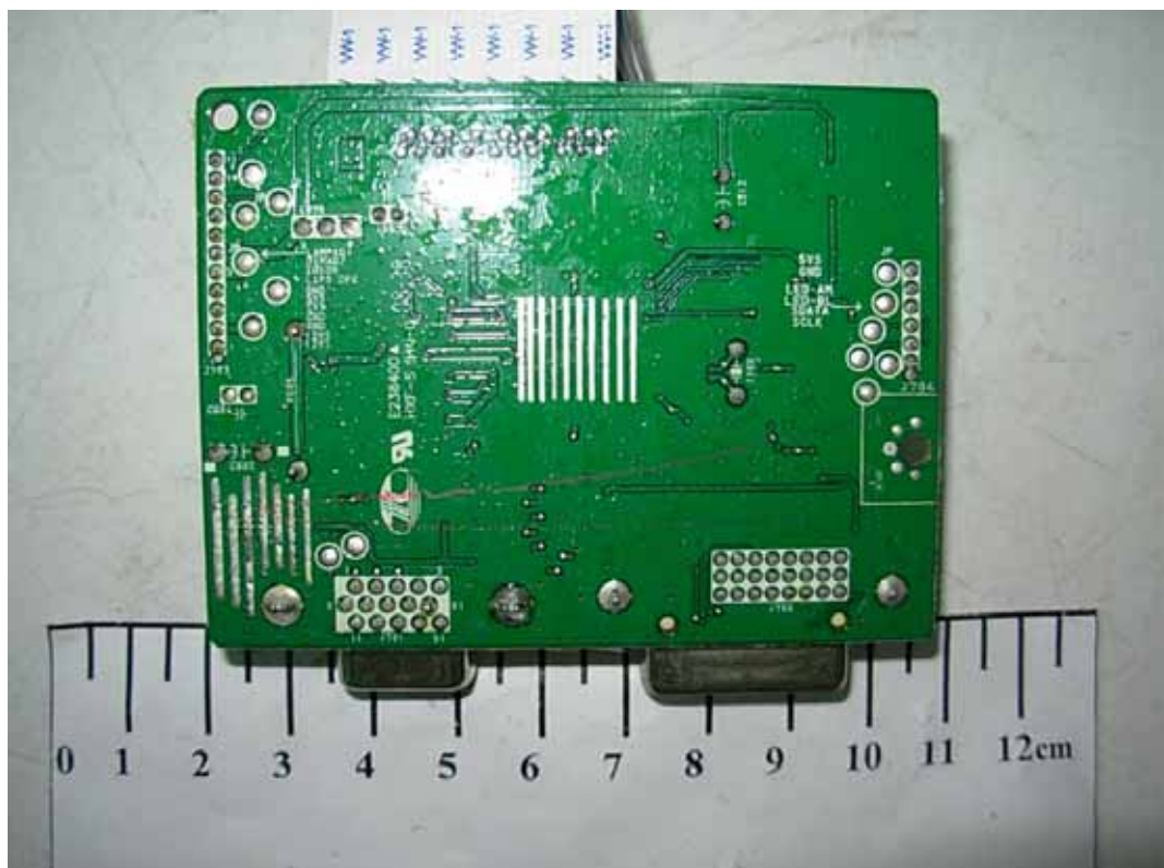
FIGURE 5 LCD MONITOR (M/N: W2044TV) MAIN BOARD (SOLDERED SIDE)
