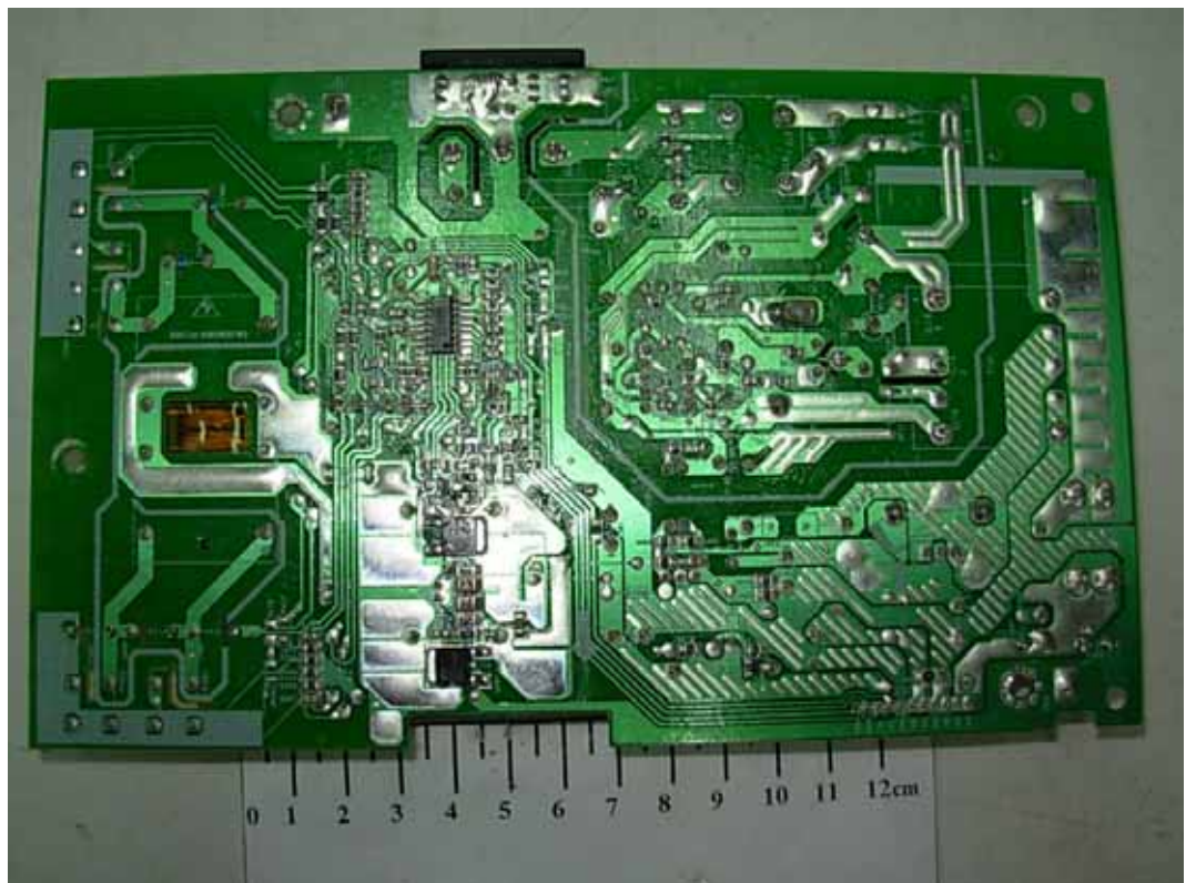
FIGURE 9 LCD MONITOR (M/N: W2044TV) POWER BOARD (SOLDERED SIDE)
