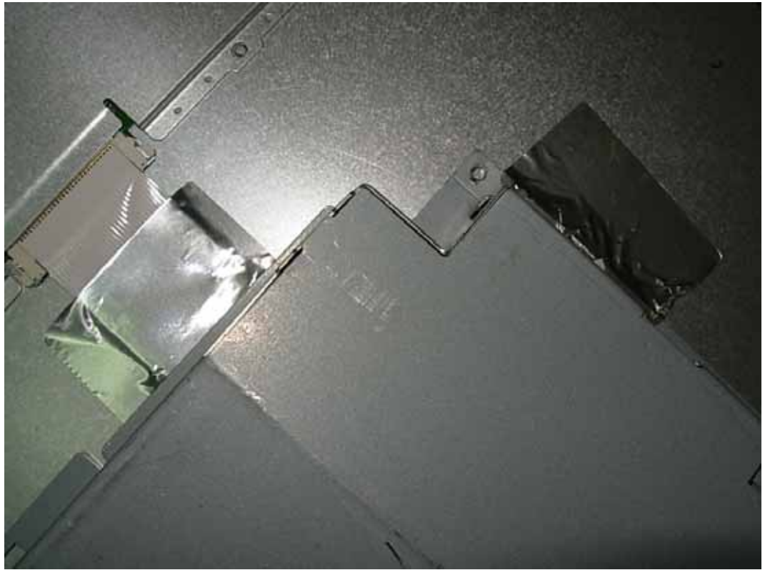
FIGURE 13 LCD MONITOR (M/N: W2044TV) DEBUG #1
