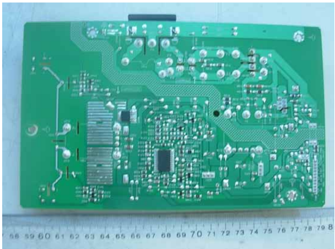
FIGURE 7 LCD MONITOR (M/N: W2043SEV) POWER BOARD (SOLDERED SIDE)
