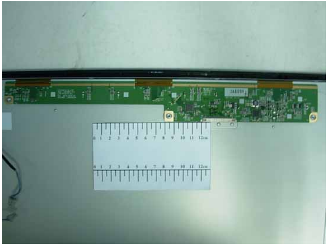
FIGURE 11 LCD MONITOR (M/N: W1954SEV) LCD PANEL MAIN BOARD (COMPONENT SIDE)
