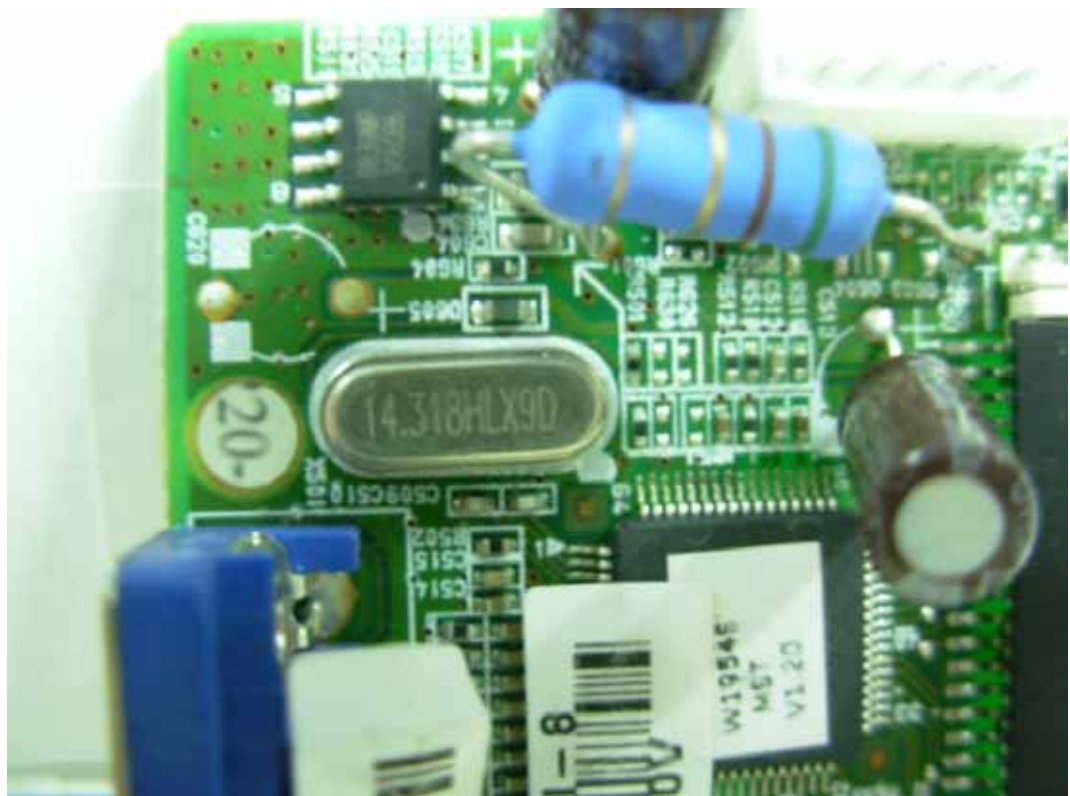
FIGURE 7 LCD MONITOR (M/N: W1954SEV) CRYSTAL ON MAIN BOARD
