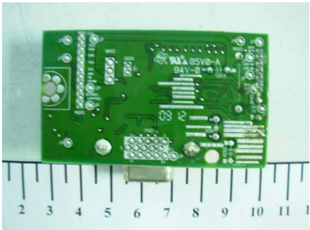
FIGURE 5 LCD MONITOR (M/N: W1954SEV) MAIN BOARD (SOLDERED SIDE)
