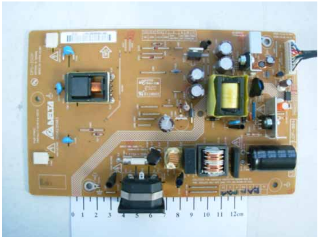
FIGURE 8 LCD MONITOR (M/N: W1954SEV) POWER BOARD (COMPONENT SIDE)
