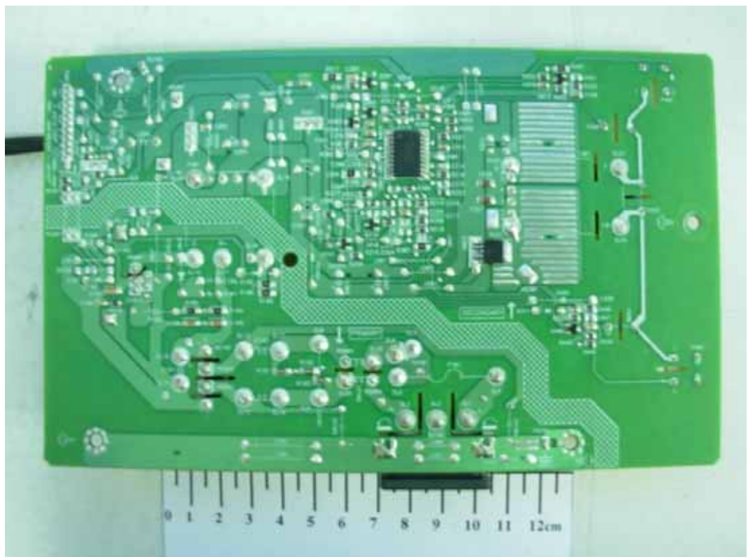
FIGURE 9 LCD MONITOR (M/N: W1954SEV) POWER BOARD (SOLDERED SIDE)
