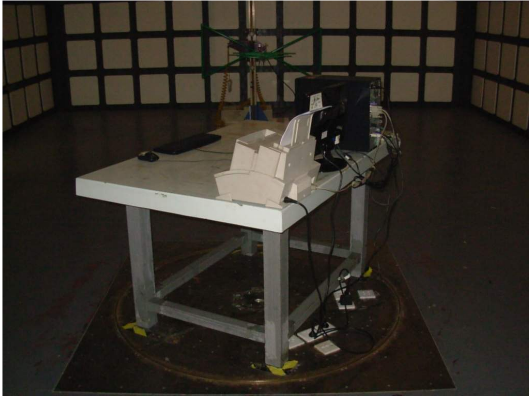
SETUP WITH MAXIMUM DETECTED EMISSION AT HORIZONTAL POLARIZATION (M/N: W1953TV, D-SUB 1280*1024@75Hz)
