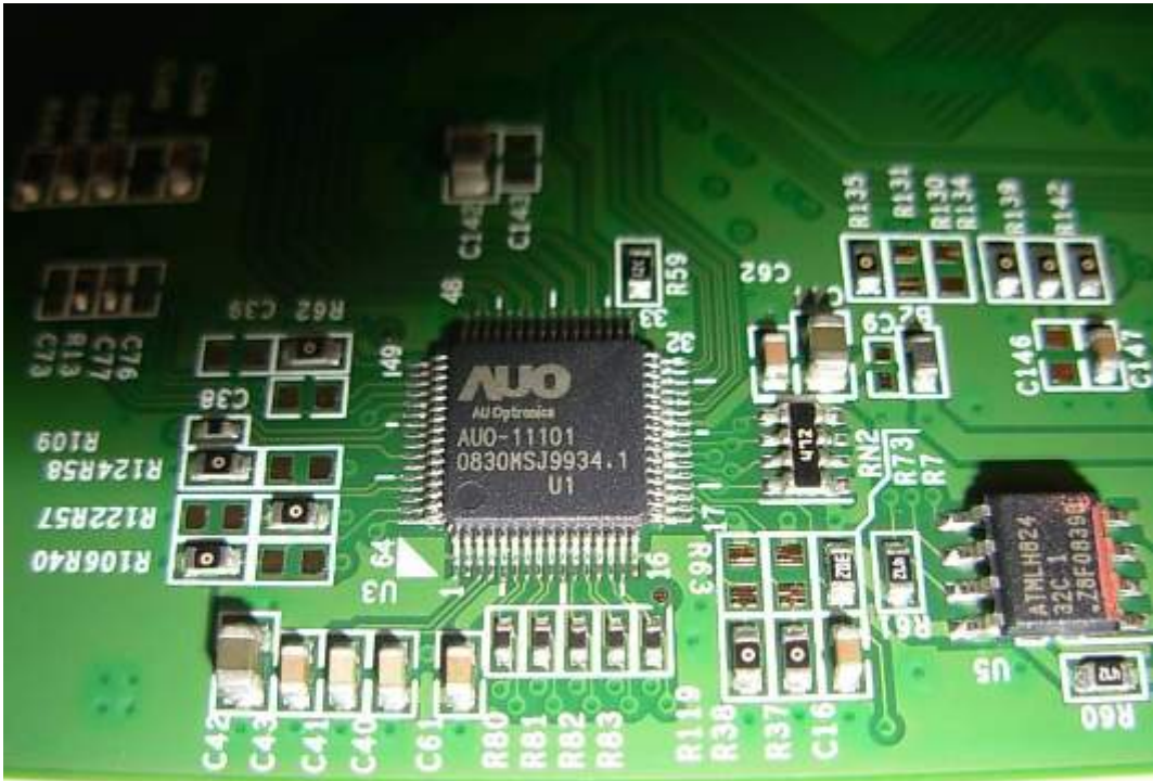
FIGURE 14 LCD MONITOR (M/N: W1953TV) CHIP ON LCD PANEL MAIN BOARD
