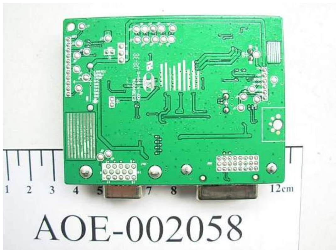
FIGURE 7 LCD MONITOR (M/N: W1953TV) MAIN BOARD (SOLDERED SIDE)
