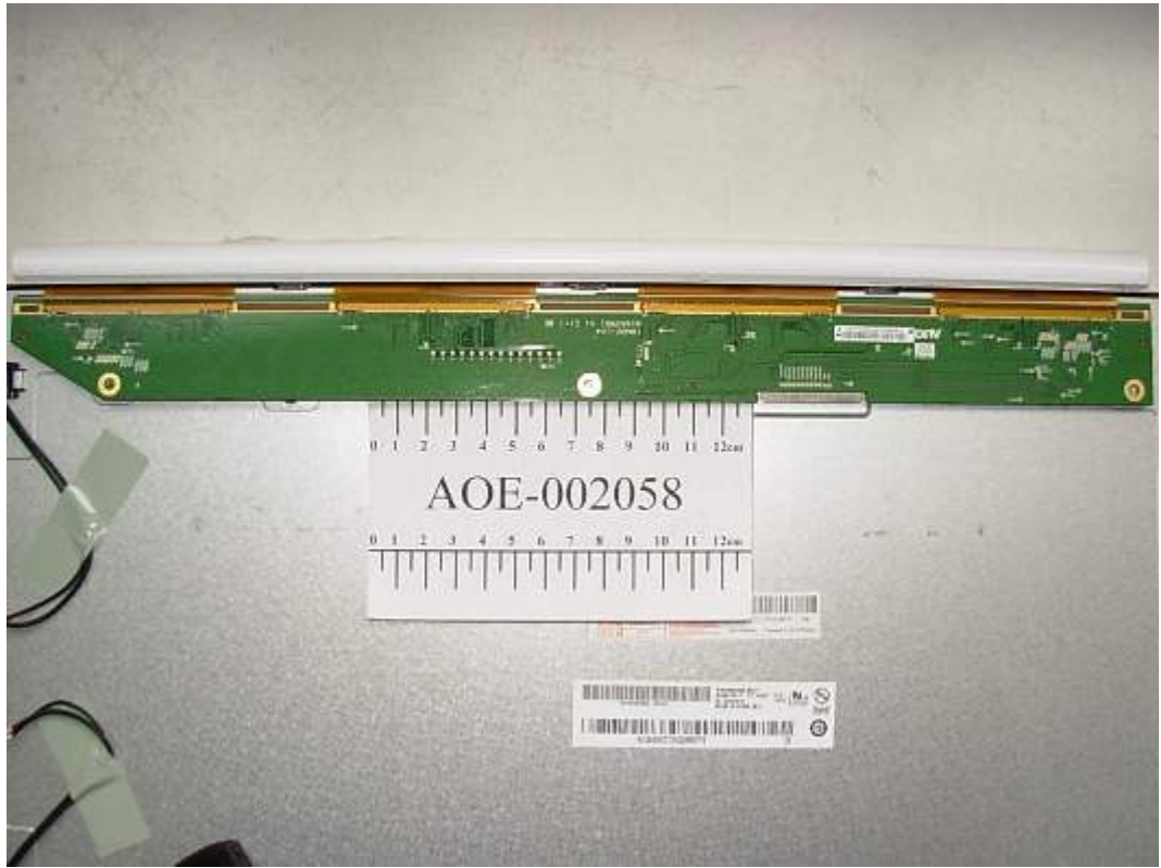
FIGURE 12 LCD MONITOR (M/N: W1953TV) LCD PANEL MAIN BOARD (COMPONENT SIDE)
