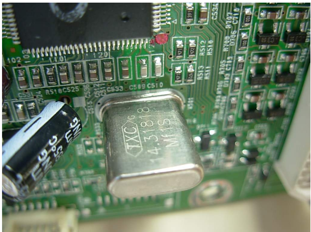
FIGURE 12 LCD MONITOR (M/N: W1952TQT) CRYSTAL ON MAIN BOARD
