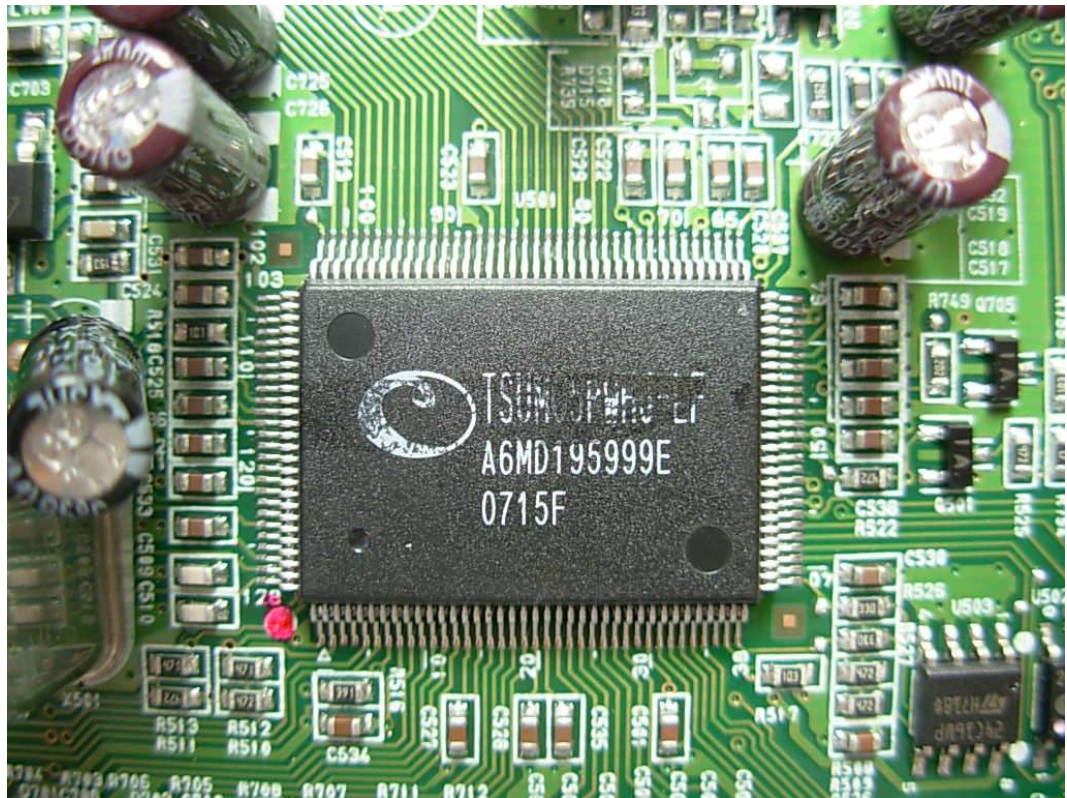
FIGURE 11 LCD MONITOR (M/N: W1952TQT) CHIP ON MAIN BOARD
