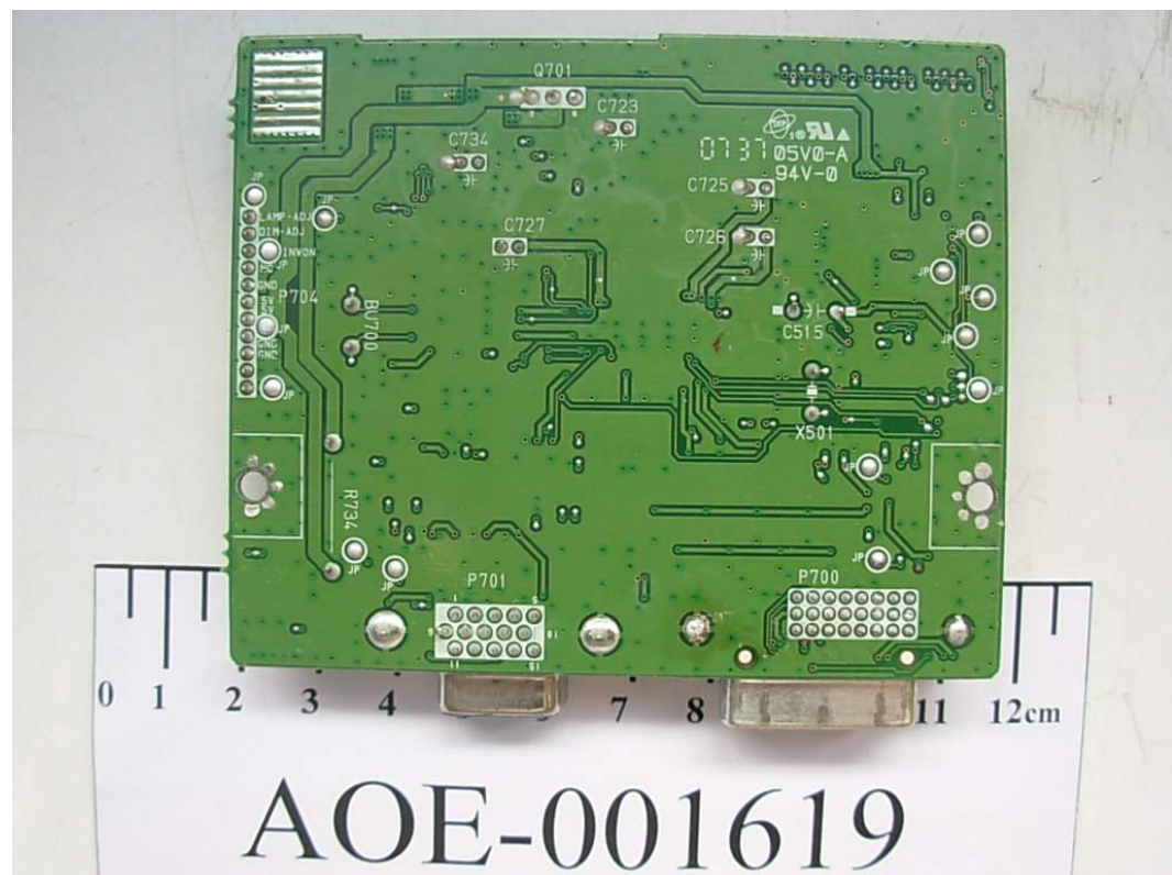
FIGURE 10 LCD MONITOR (M/N: W1952TQT) MAIN BOARD (SOLDERED SIDE)
