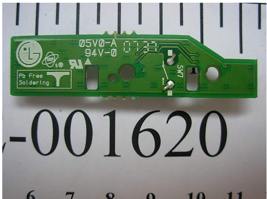
FIGURE 23 LCD MONITOR (M/N: W1952SQT) LED BOARD (BACK VIEW)
