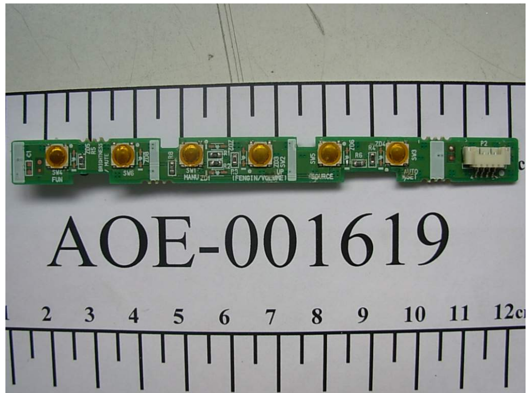
FIGURE 5 LCD MONITOR (M/N: W1952TQT) BUTTON BOARD (FRONT VIEW)
