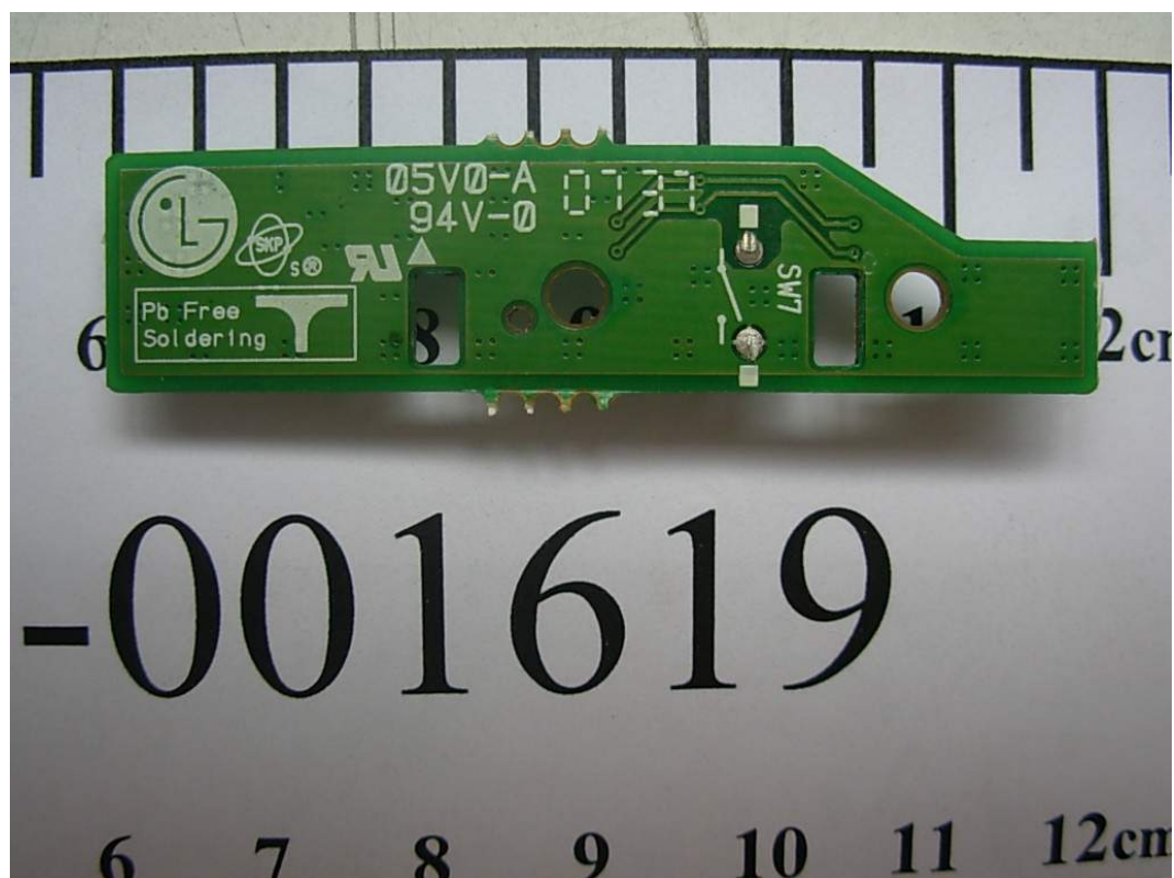
FIGURE 4 LCD MONITOR (M/N: W1952TQT) LED BOARD (BACK VIEW)
