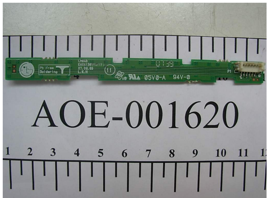
FIGURE 25 LCD MONITOR (M/N: W1952SQT) BUTTON BOARD (BACK VIEW)
