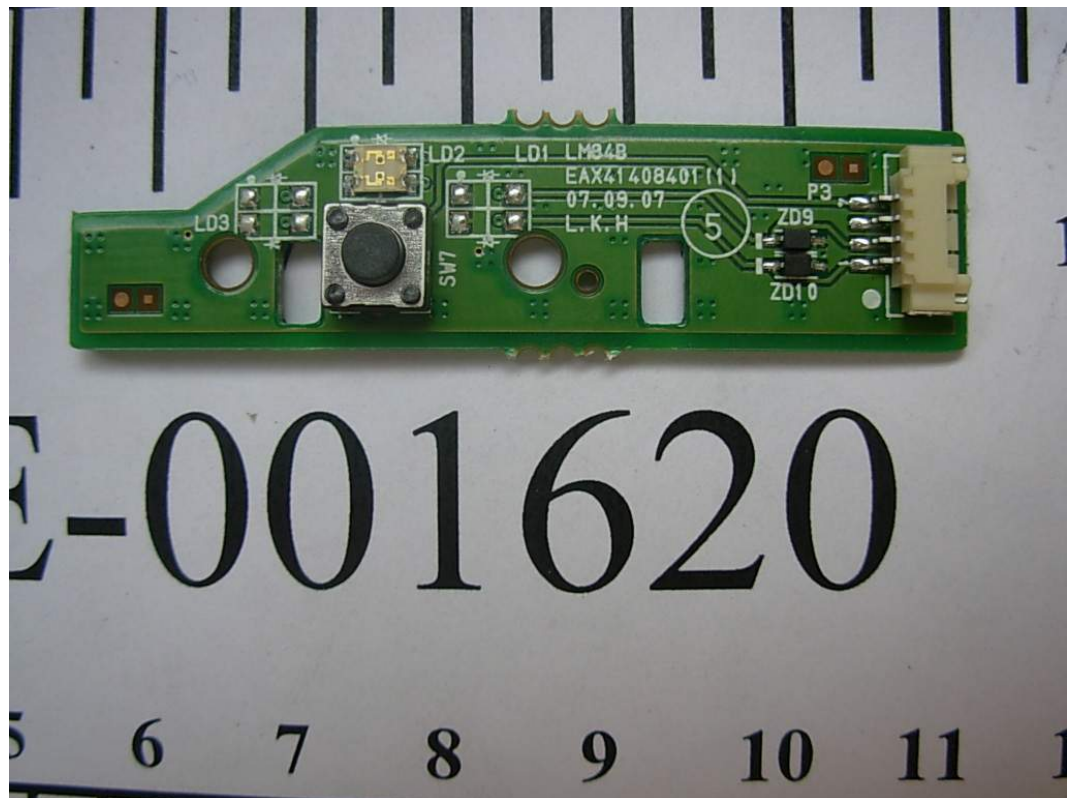
FIGURE 22 LCD MONITOR (M/N: W1952SQT) LED BOARD (FRONT VIEW)
