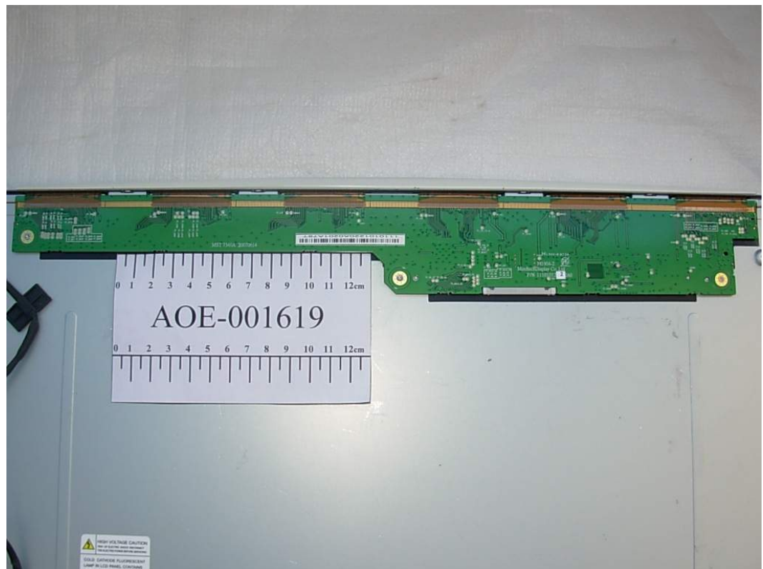
FIGURE 15 LCD MONITOR (M/N: W1952TQT) LCD PANEL MAIN BOARD (FRONT VIEW)
