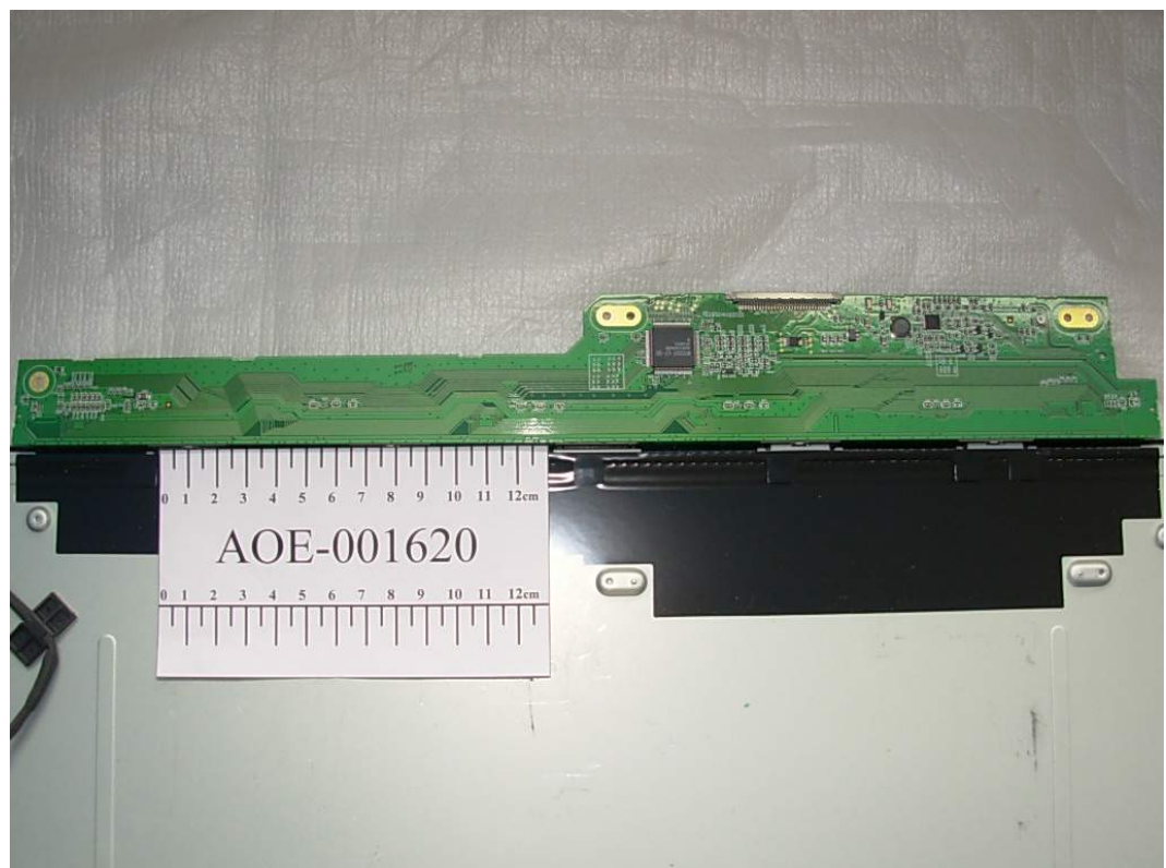
FIGURE 35 LCD MONITOR (M/N: W1952SQT) LCD PANEL MAIN BOARD (BACK VIEW)
