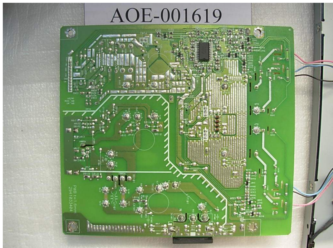
FIGURE 8 LCD MONITOR (M/N: W1952TQT) POWER BOARD (SOLDERED SIDE)
