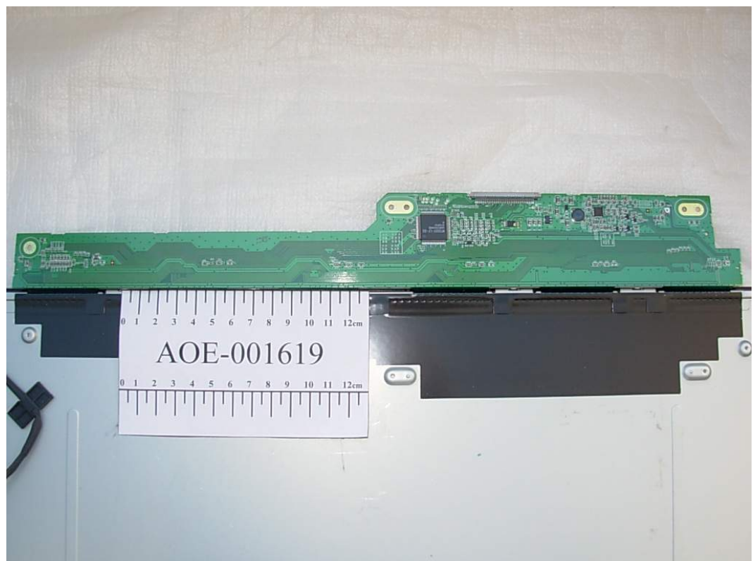
FIGURE 16 LCD MONITOR (M/N: W1952TQT) LCD PANEL MAIN BOARD (BACK VIEW)
