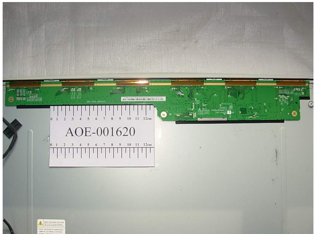
FIGURE 34 LCD MONITOR (M/N: W1952SQT) LCD PANEL MAIN BOARD (FRONT VIEW)
