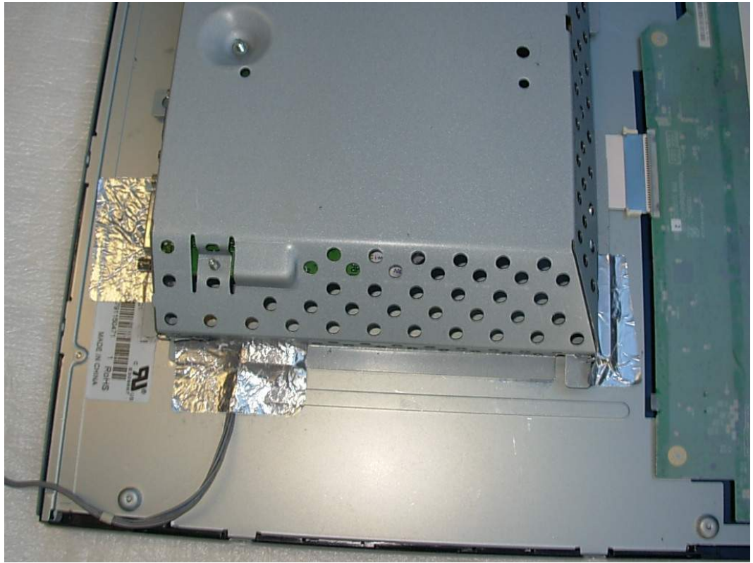
FIGURE 19 LCD MONITOR (M/N: W1952TQT) DEBUG 2
