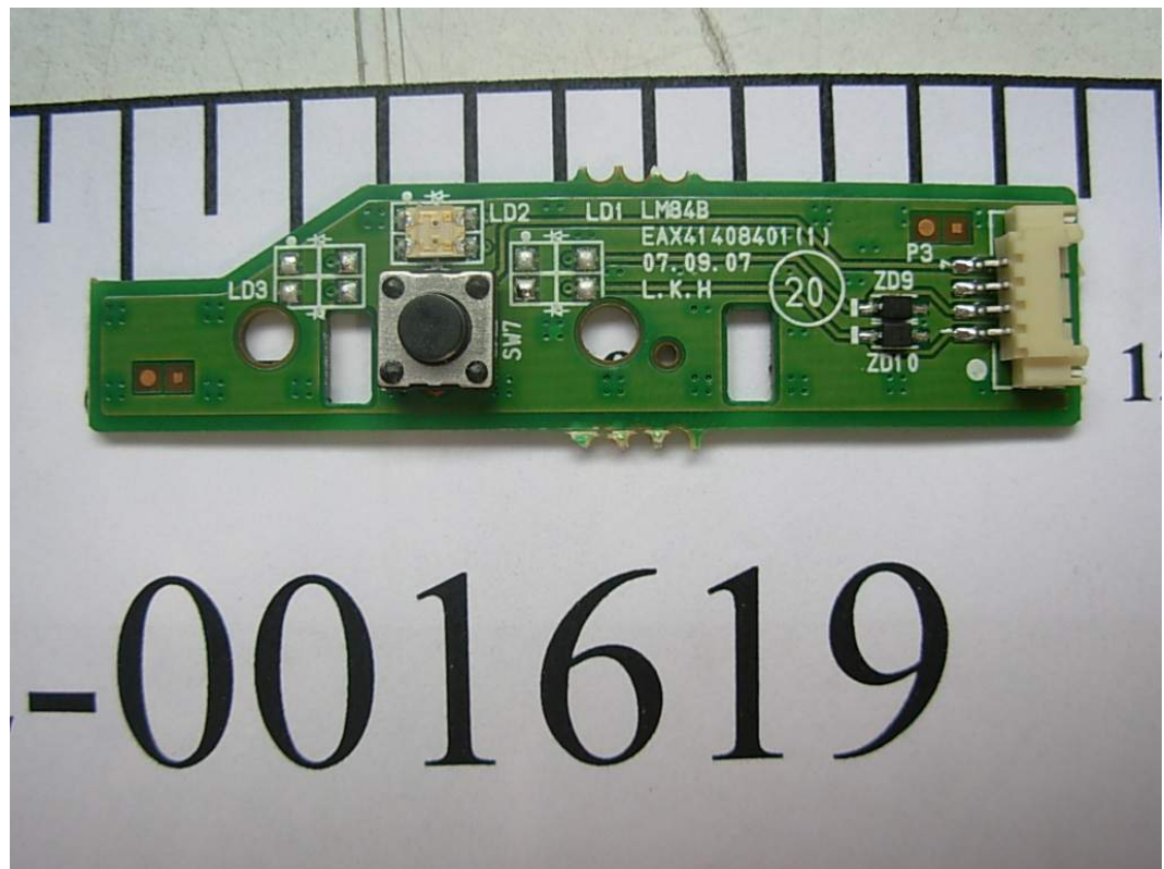
FIGURE 3 LCD MONITOR (M/N: W1952TQT) LED BOARD (FRONT VIEW)
