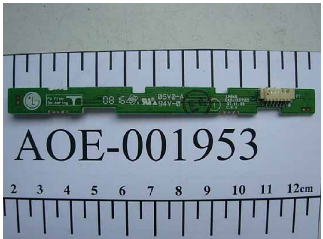
FIGURE 3 LCD MONITOR (M/N: W1952TET) KEY BOARD (SOLDERED SIDE)
