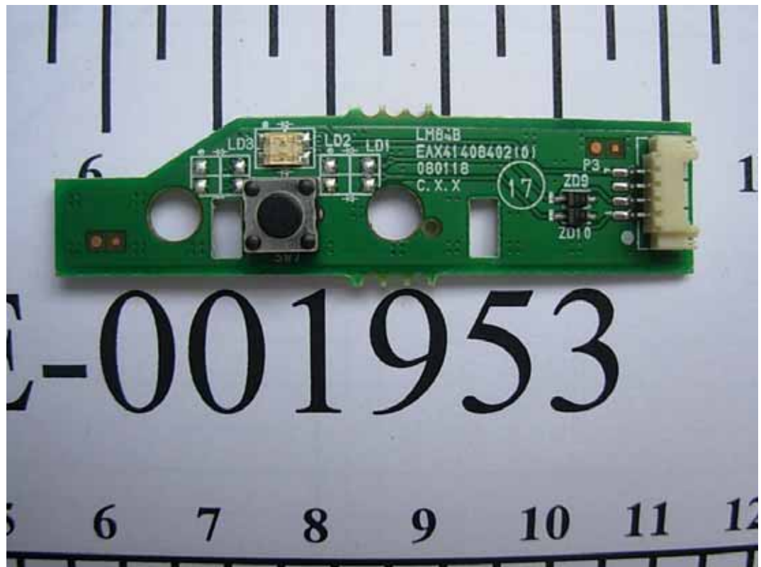
FIGURE 4 LCD MONITOR (M/N: W1952TET) LED BOARD (COMPONENT SIDE)
