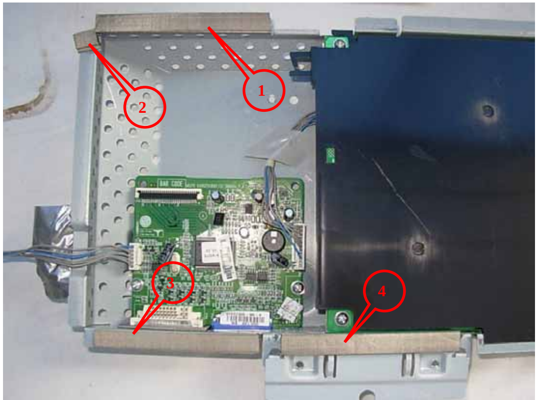
FIGURE 21 LCD MONITOR (M/N: W1952TET) DEBUG 3
