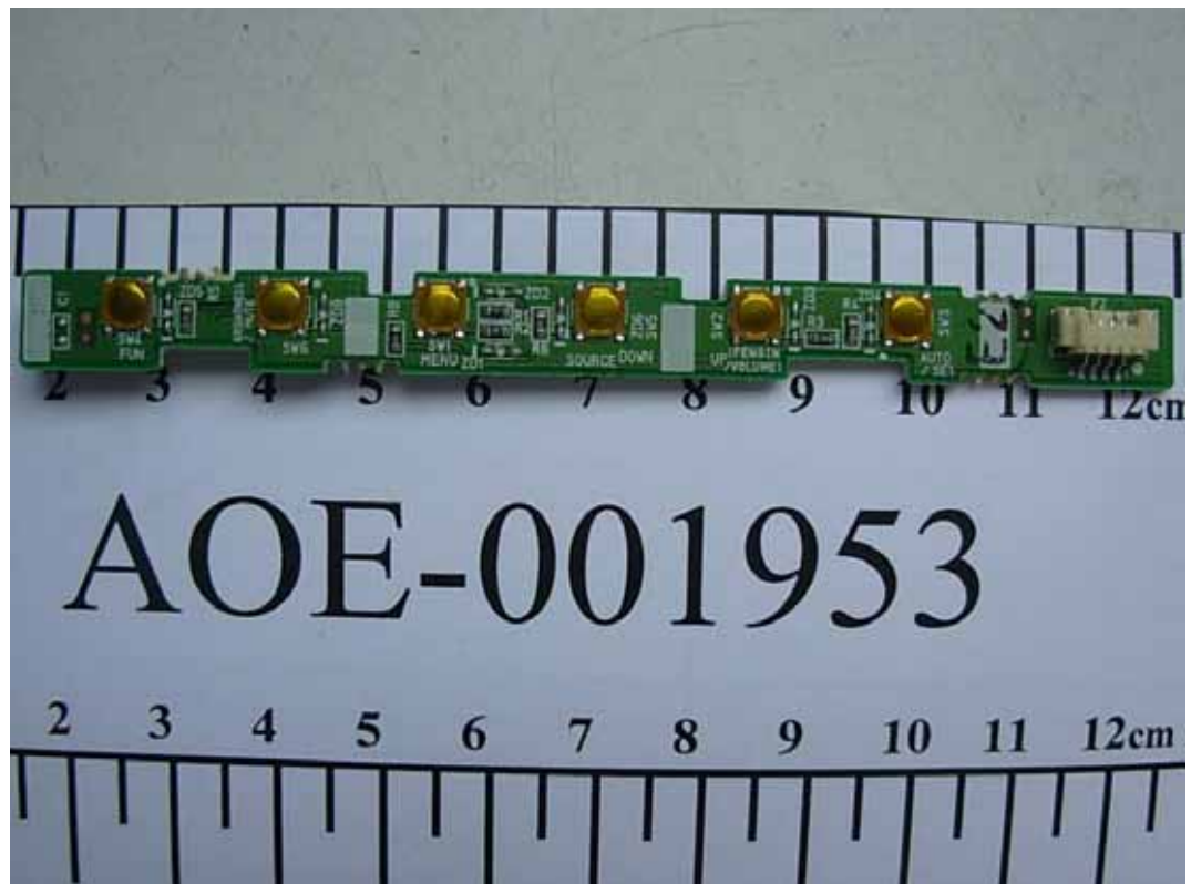
FIGURE 2 LCD MONITOR (M/N: W1952TET) KEY BOARD (COMPONENT SIDE)
