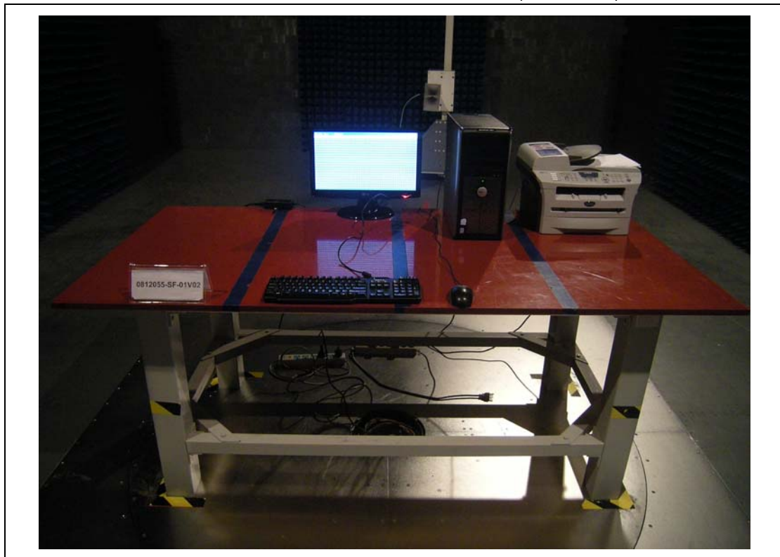
Front View of Radiated Emission Test (Above 1G)
