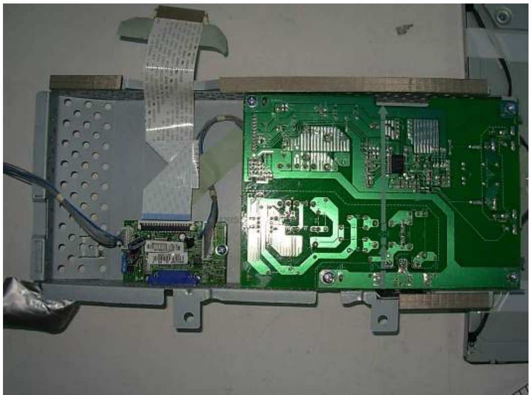
FIGURE 18 LCD MONITOR (M/N: W1941ST) DEBUG #2
