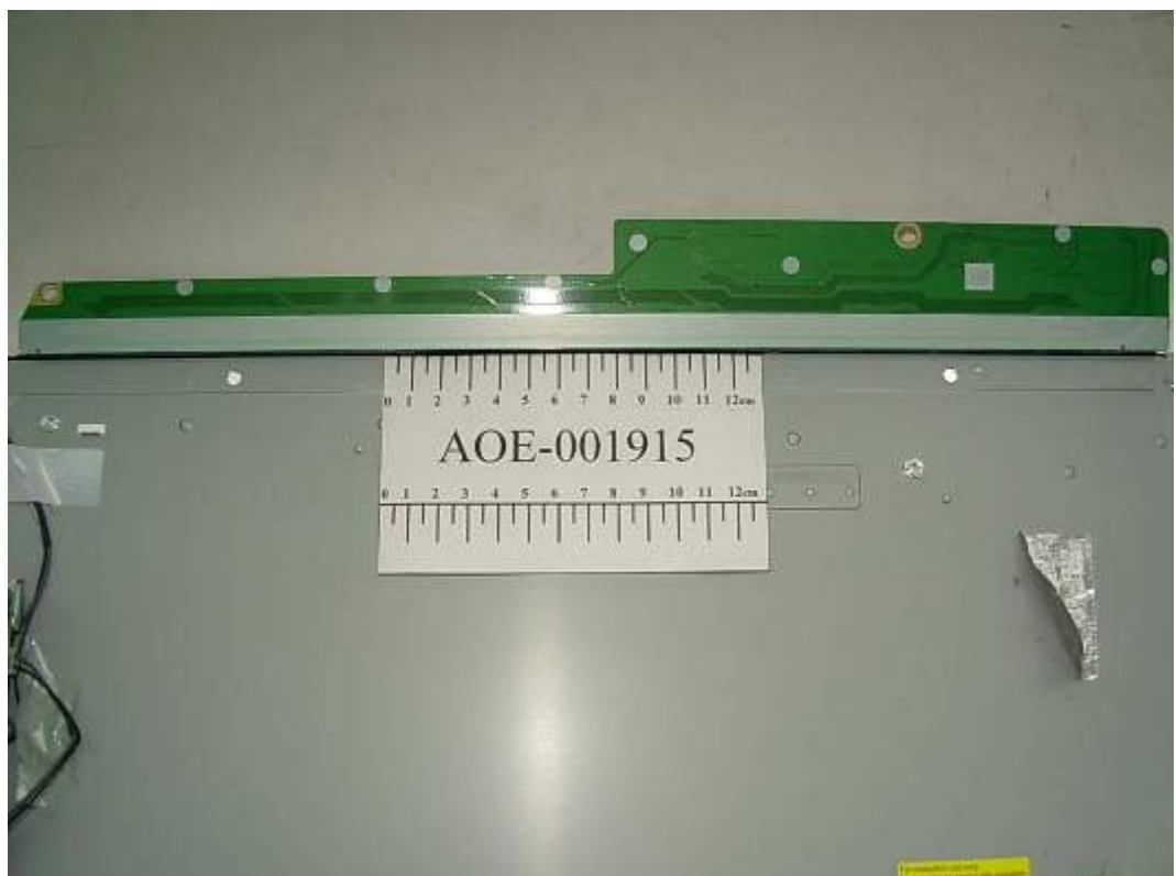
FIGURE 14 LCD MONITOR (M/N: W1941ST) LCD PANEL MAIN BOARD (SOLDERED SIDE)
