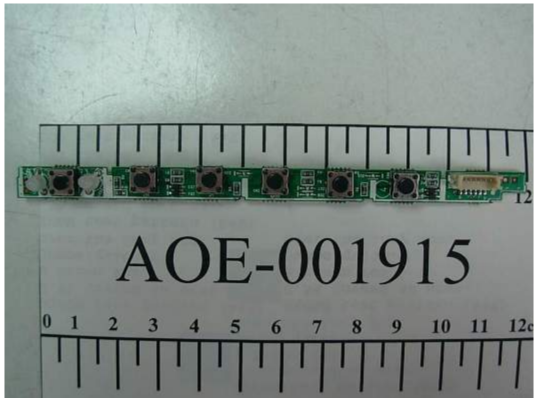
FIGURE 3 LCD MONITOR (M/N: W1941ST) KEY BOARD (COMPONENT SIDE)
