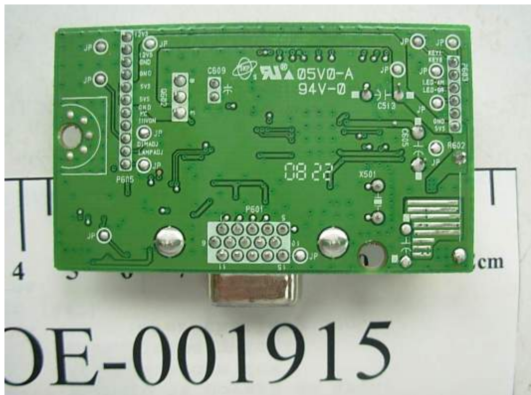
FIGURE 6 LCD MONITOR (M/N: W1941ST) MAIN BOARD (SOLDERED SIDE)
