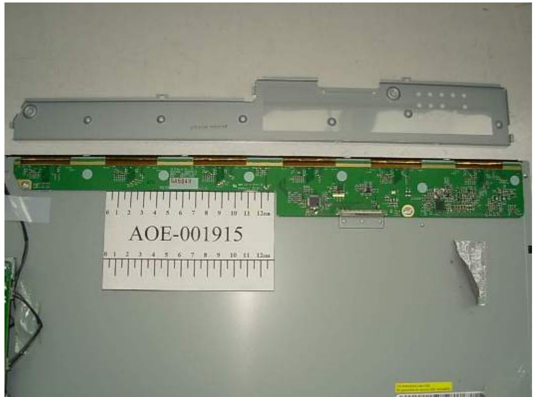
FIGURE 12 LCD MONITOR (M/N: W1941ST) LCD PANEL MAIN BOARD SHIELDED SHELL REMOVED
