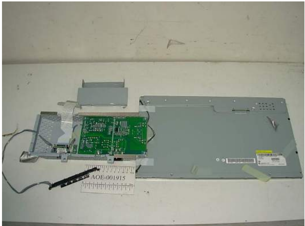
FIGURE 2 LCD MONITOR (M/N: W1941ST) BOARDS REMOVED
