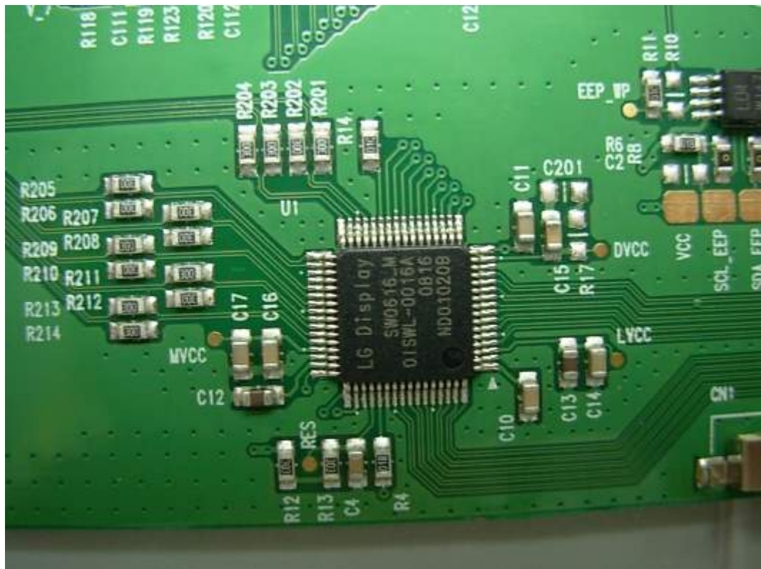
FIGURE 15 LCD MONITOR (M/N: W1941ST) CHIP ON LCD PANEL MAIN BOARD
