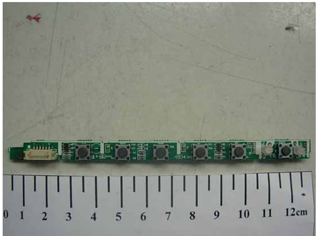
FIGURE 3 LCD MONITOR (M/N: W1941JT) KEYBOARD (COMPONENT SIDE)
