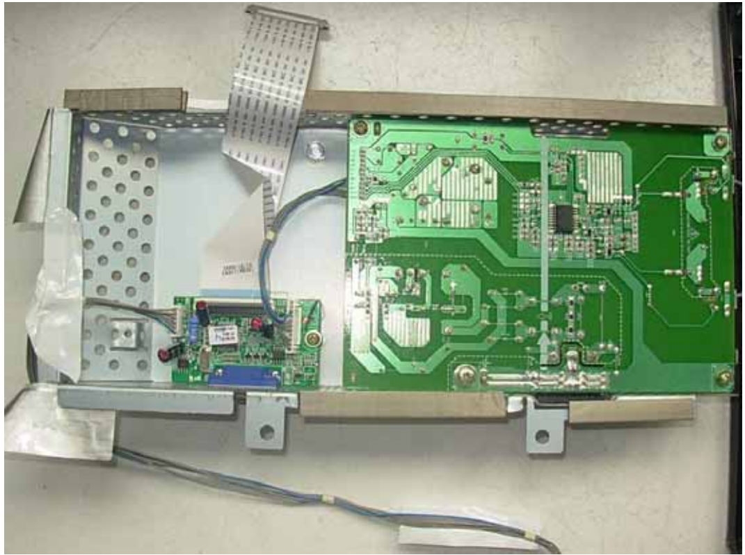
FIGURE 16 LCD MONITOR (M/N: W1941JT) DEBUG #2
