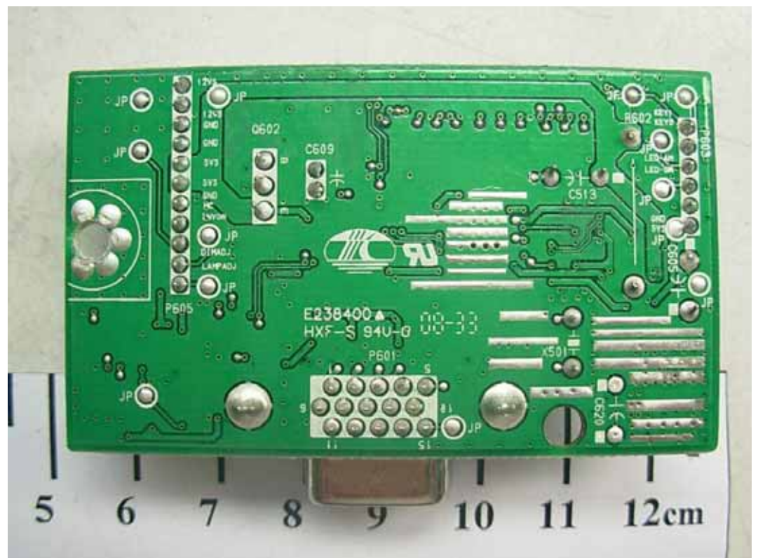
FIGURE 6 LCD MONITOR (M/N: W1941JT) MAIN BOARD (SOLDERED SIDE)
