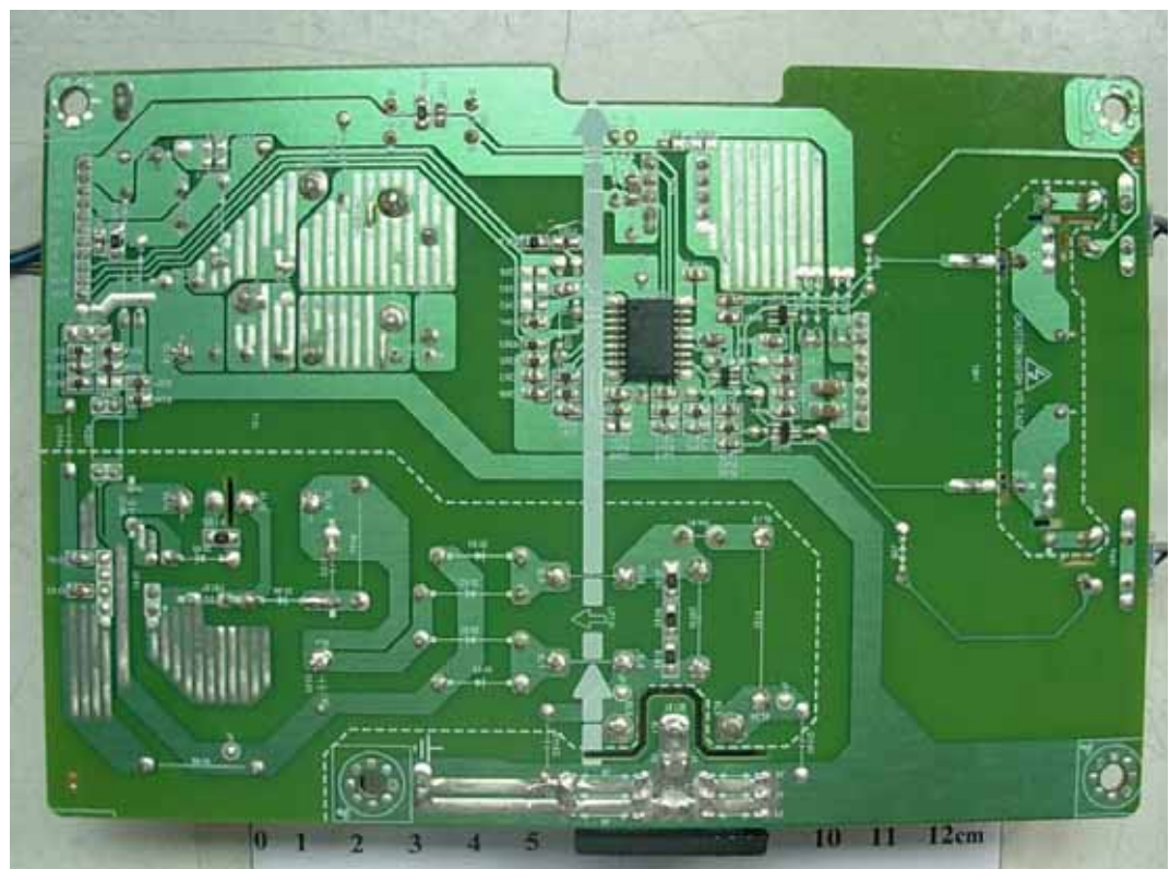
FIGURE 9 LCD MONITOR (M/N: W1941JT) POWER BOARD (SOLDERED SIDE)
