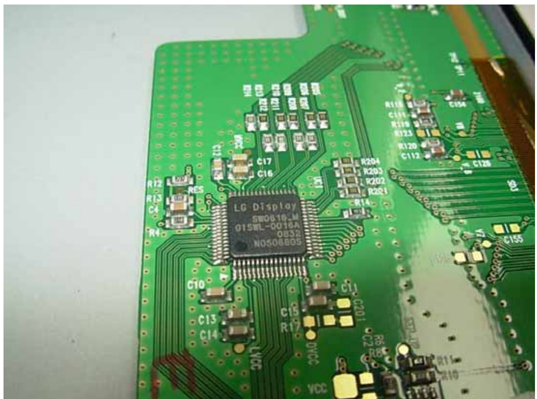
FIGURE 13 LCD MONITOR (M/N: W1941JT) CHIP ON LCD PANEL MAIN BOARD
