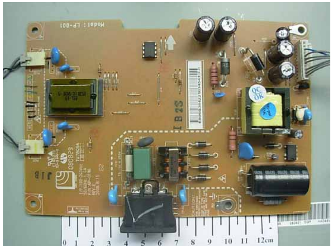
FIGURE 8 LCD MONITOR (M/N: W1941JT) POWER BOARD (COMPONENT SIDE)
