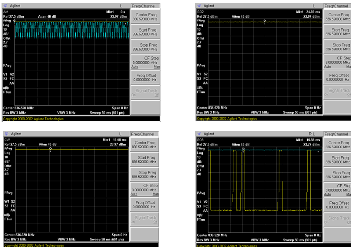
Figure 25 Zero-Span Plots
