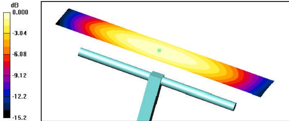
0 dB = 0.444A/m
