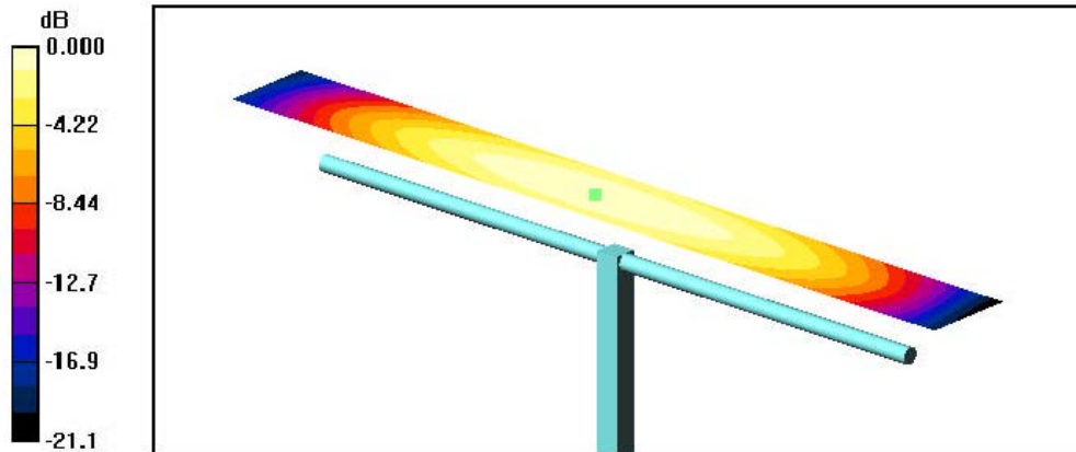
0 dB = 0.482A/m
