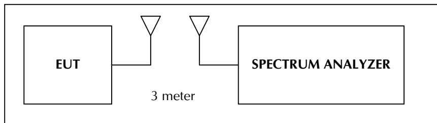
Figure A-1. Test Instrument & Measurement Setup
