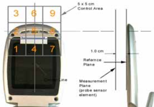
Figure 13 E/H-Field Emissions Test Setup Diagram
