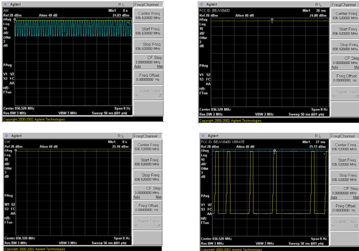
Figure 26 Zero-Span Plots
