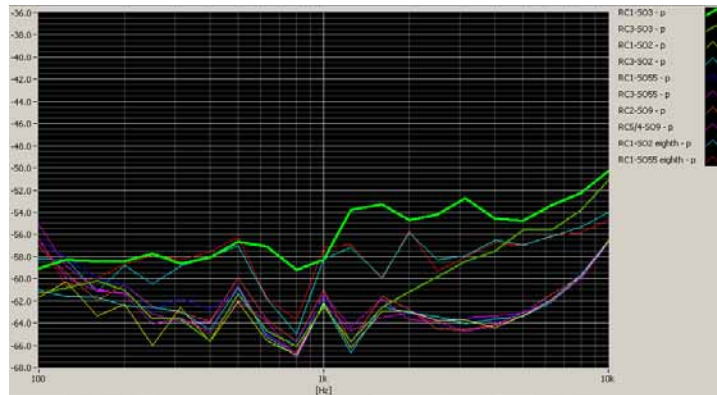
Figure 7-1 CDMA2000 Audio Band Magnetic Noise
