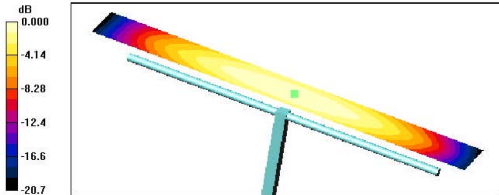
0 dB = 0.495A/m
