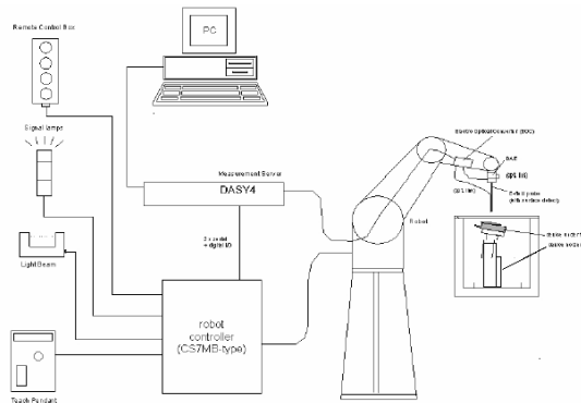
Figure 9 SPEAG Robotic System Diagram
