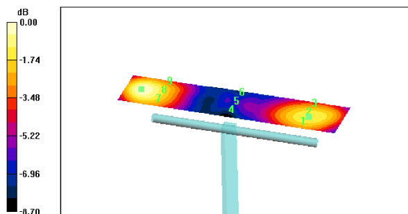
0 dB = 169.5V/m
