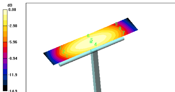
0 dB = 0.466A/m
