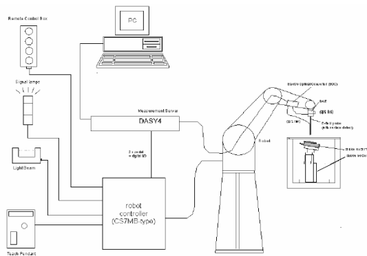
Figure 7 SPEAG Robotic System Diagram
