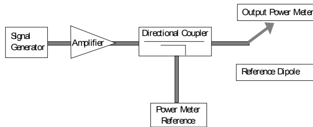
Figure 11 Setup for Desired Output Power to Dipole
