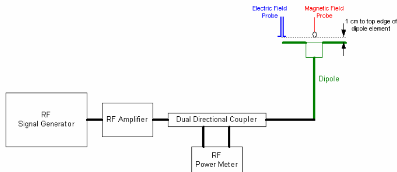
Figure 13 System Check Setup
