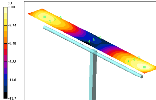
0 dB = 198.4V/m
