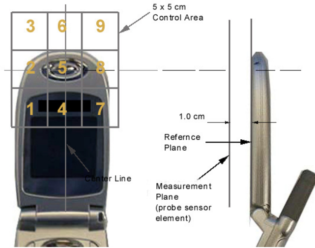
Figure 8 E/H-Field Emissions Test Setup Diagram
