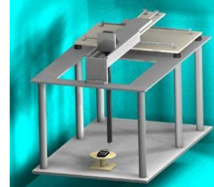
Figure 4 RF Near-Field Scanner
