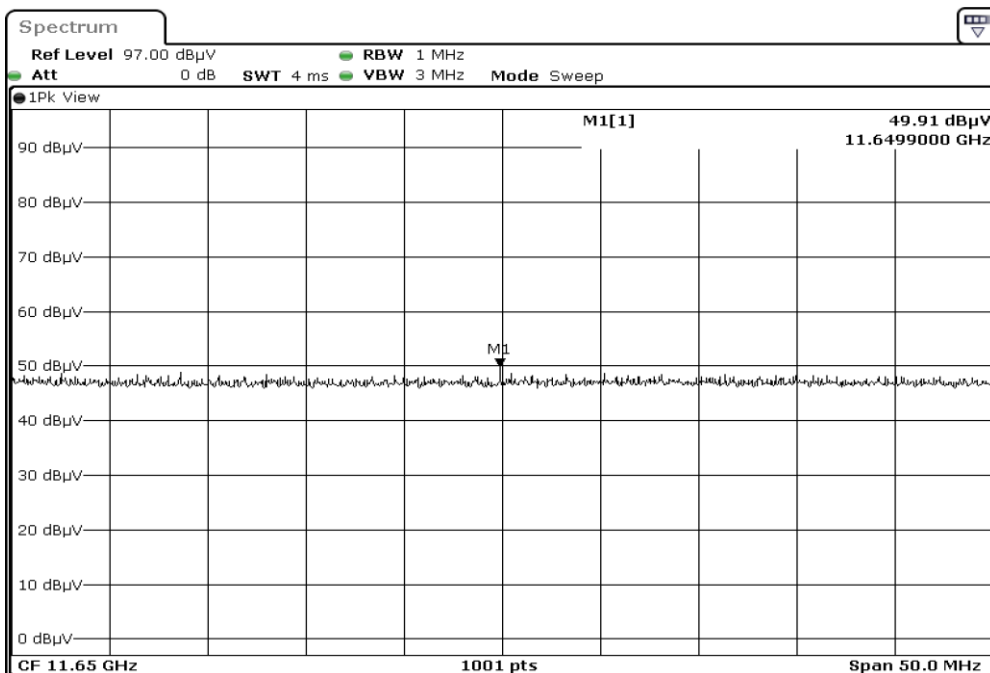
F3 X2 11650.0 Harmonic Horizontal PEAK
