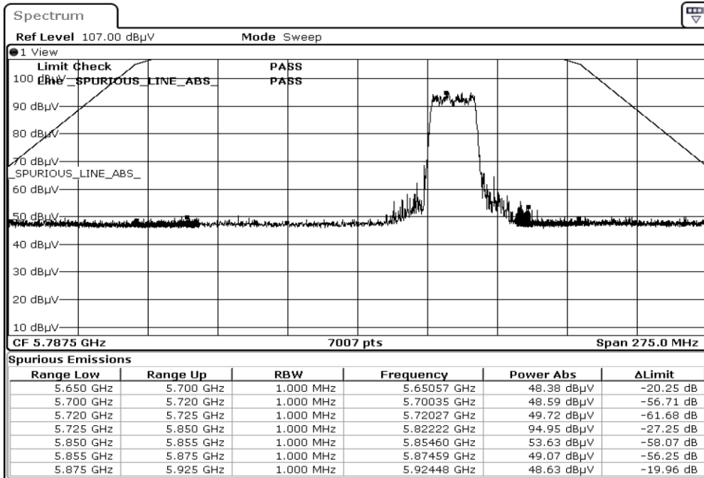
5825.0 F3 RestrictedBand Horizontal PEAK
