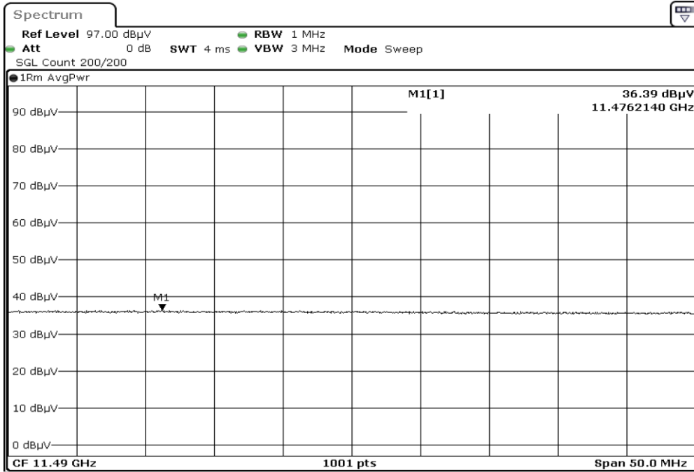
F1 X2 11490.0 Harmonic Vertical AVG
