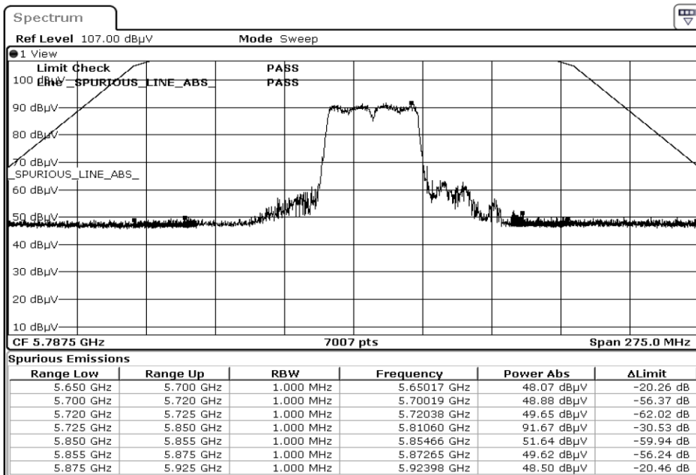
5795.0 F3 RestrictedBand Vertical PEAK
