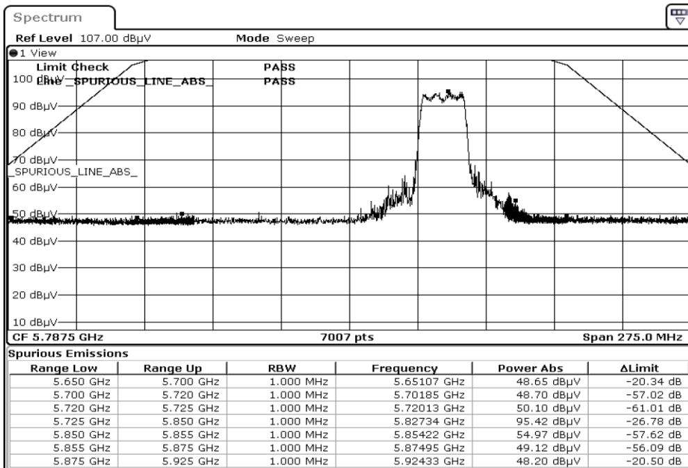
5825.0 F3 RestrictedBand Vertical PEAK
