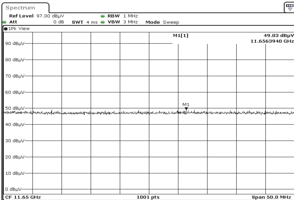
F3 X2 11650.0 Harmonic Vertical PEAK
