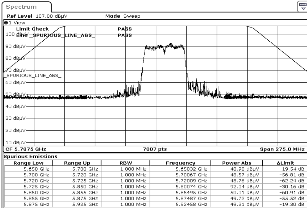
5795.0 F3 RestrictedBand Horizontal PEAK
