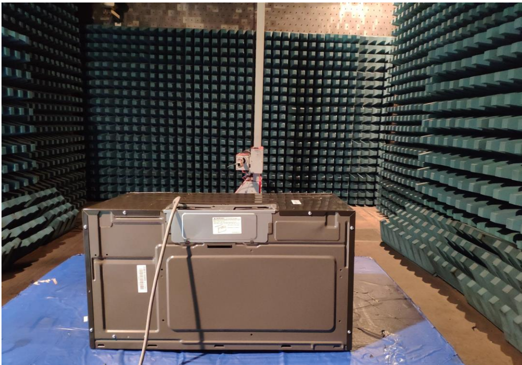
Radiated Emission (18GHz ~ 25GHz)
