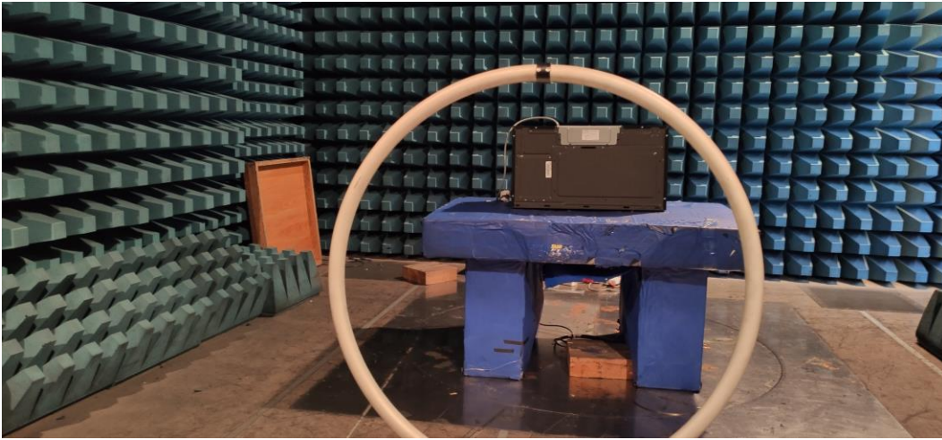
Radiated Emission (9KHz ~ 30MHz)
