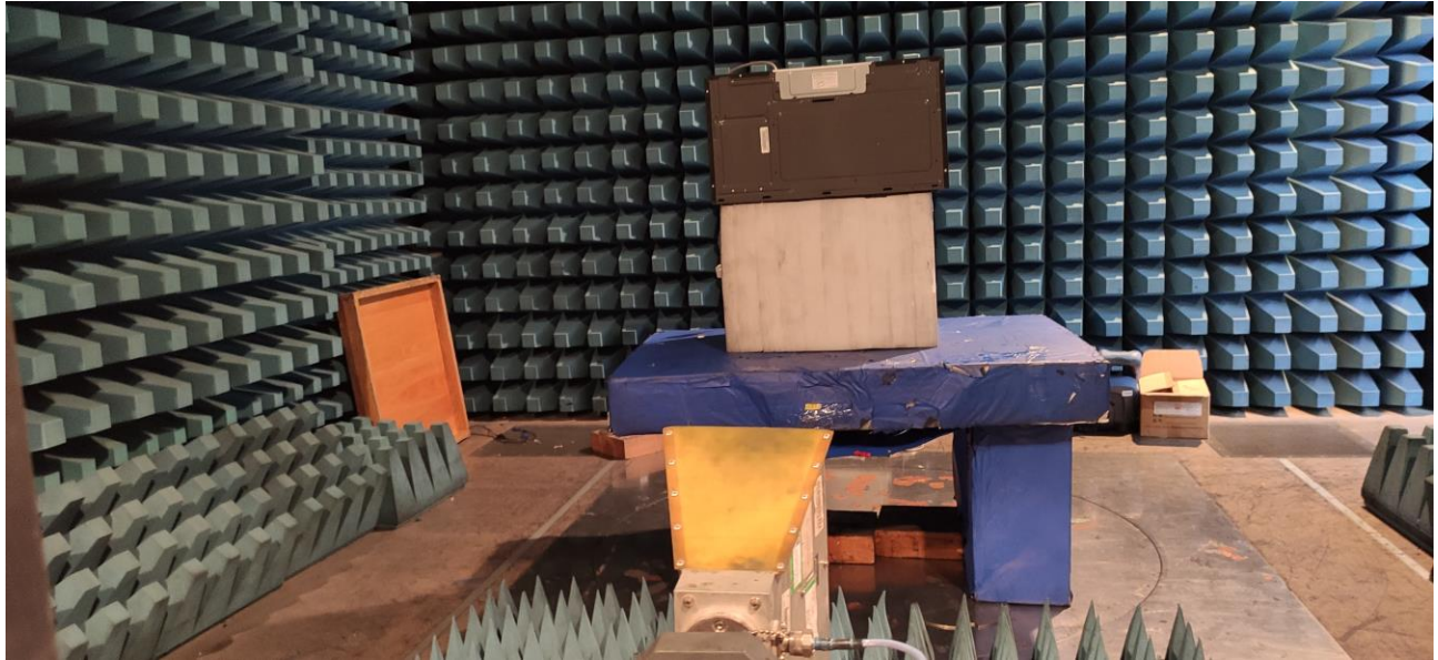
Radiated Emission (1GHz ~ 18GHz)
