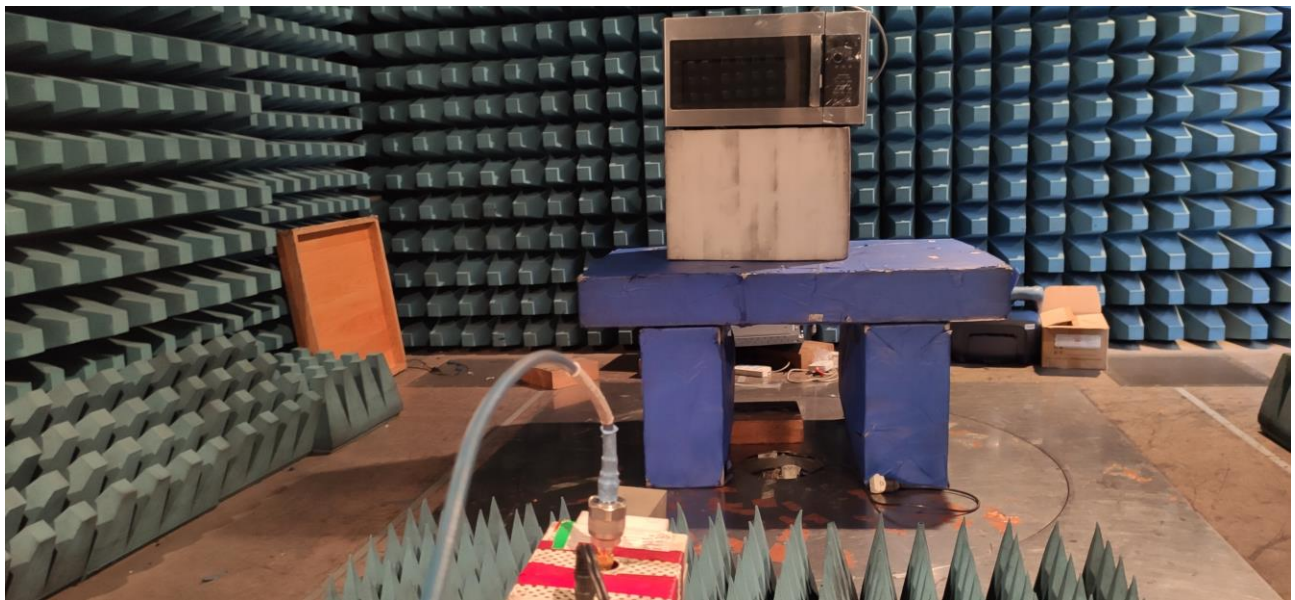
Radiated Emission (18GHz ~ 25GHz)
