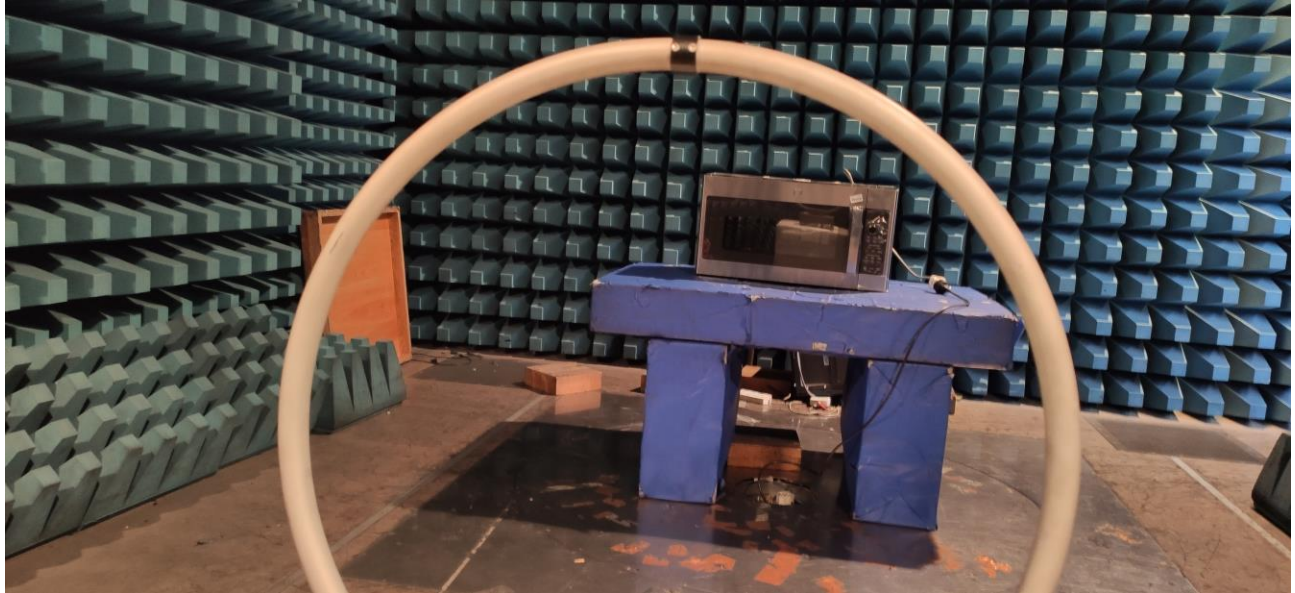
Radiated Emission (9KHz ~ 30MHz)
