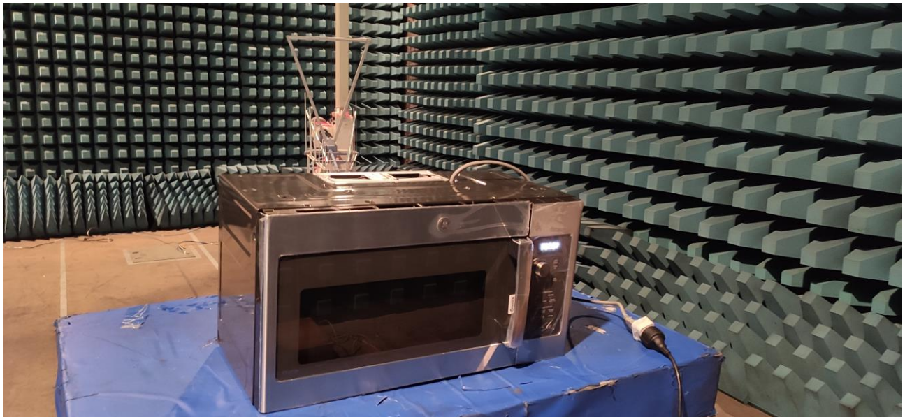
Radiated Emission (30MHz ~ 1GHz)
