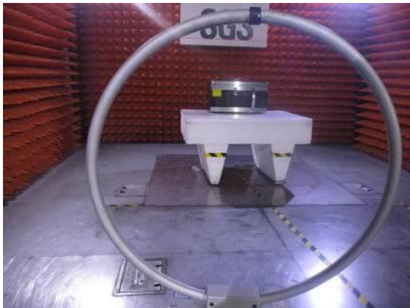
Radiated Emissions (Magnetic field Strength)(150kHz-30MHz) Test Setup
