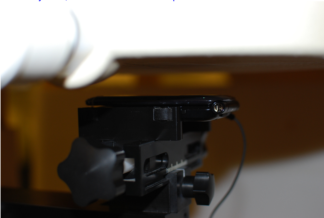
10. Body SAR, Front Side with 2.0 cm Space
