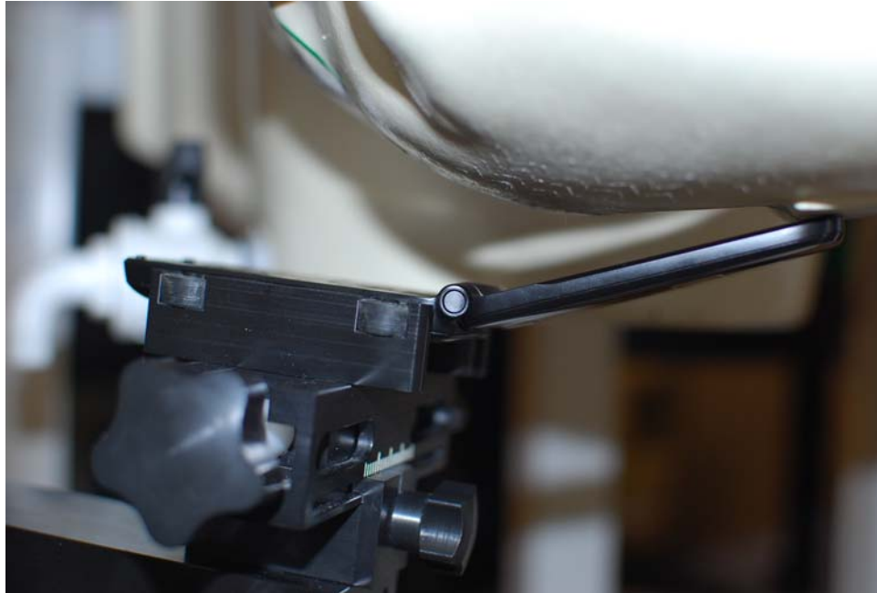
Figure 19-3 SAR Test Setup Photo 3 – Left Tilt
