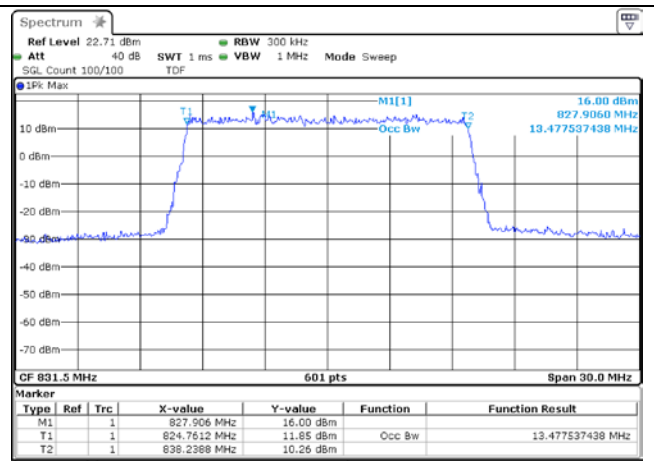
15 MHz 16QAM Low Channel – Full RB
