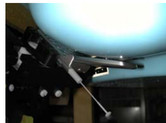
Figure 18. Head SAR Test Setup
