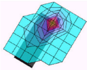
Figure 8.1 Sample SAR Area Scan
