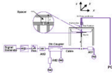
Figure 13.1 Dipole Validation Test Setup
