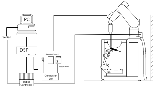
Figure 3.1 SAR Measurement System Setup
