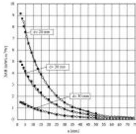
Figure 5.1 E-Field and Temperature measurements at 900MHz [7]
